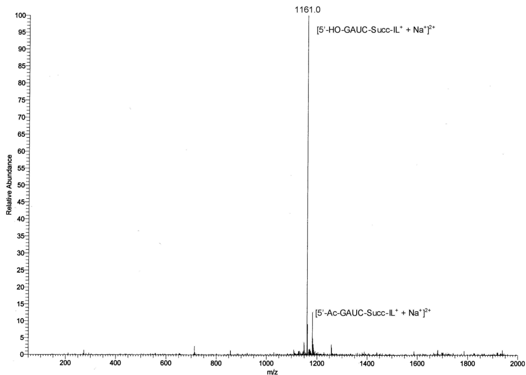
Fig. 1. Low resolution ESIMS of 9 .
