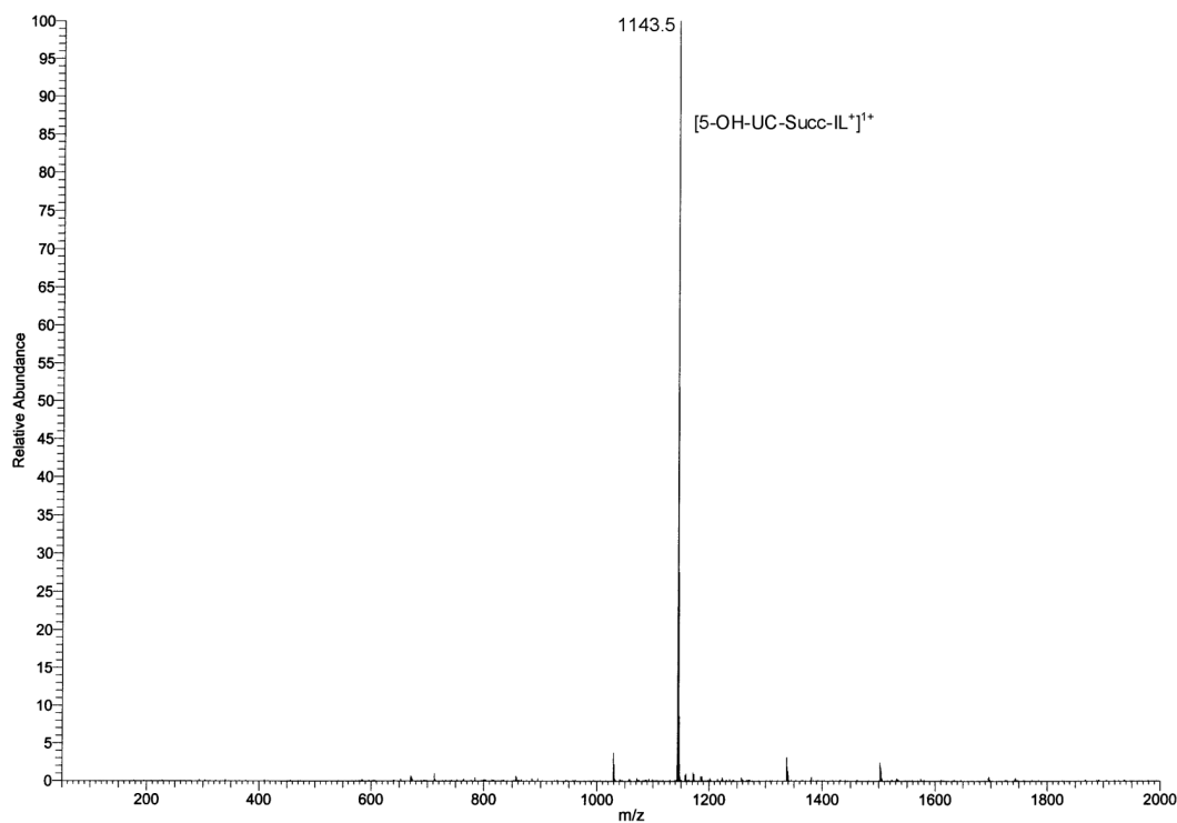
Fig. 2 Low resolution ESIMS of 3 .
