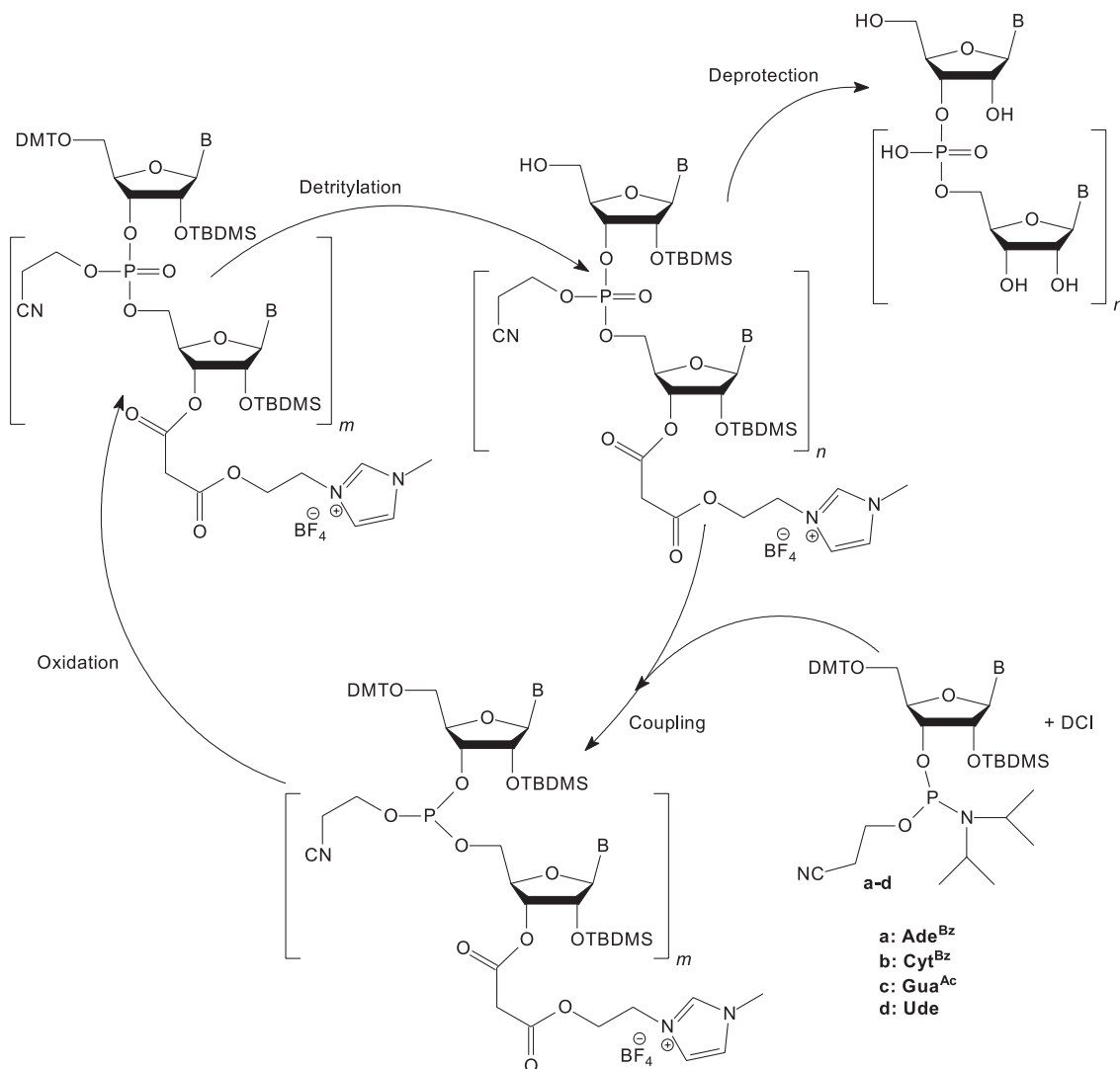
Scheme 3. Oligoribonucleotide coupling cycle (illustrated as one regioisomer).
