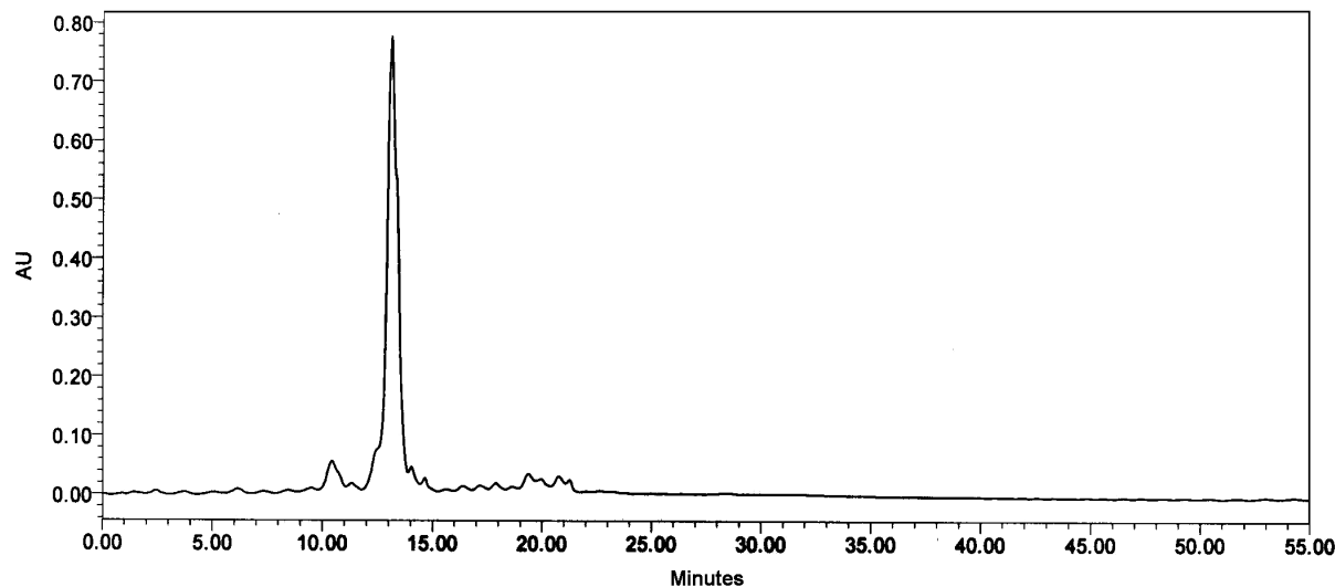
Fig. 3. HPLC chromatogram of the co-injection of 11 and solution-phase synthesized standard.
