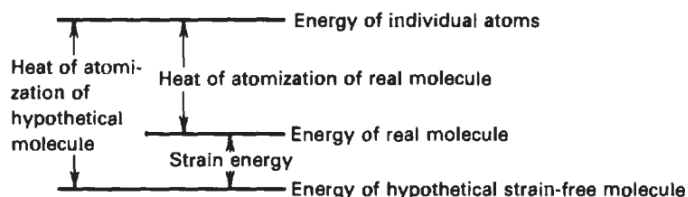
FIGURE 4.5 Strain energy calculation.
