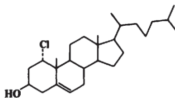
1 \alpha -Chloro-5-cholesten-3 \beta -ol
