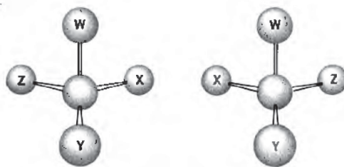
FIGURE 4.1 Enantiomers.
