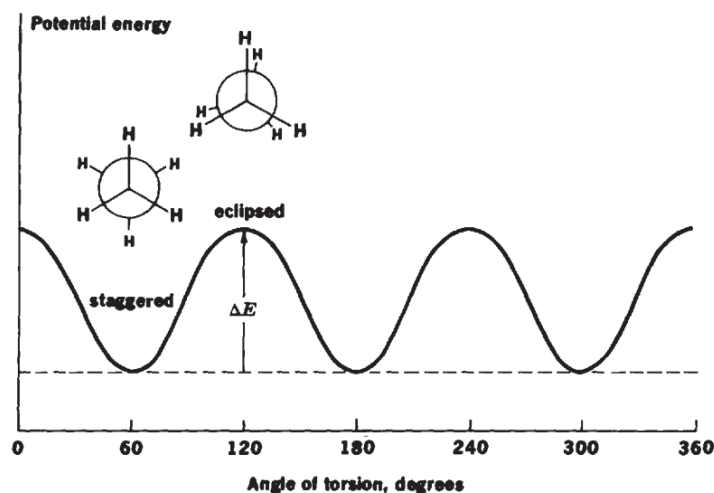
FIGURE 4.3 Conformational energy diagram for ethane.
