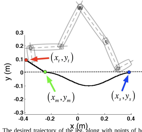
Fig. 3. The desired trajectory of the leg, along with points of heel-strike, mid-stance and toe-off used for the design of the trajectory.
