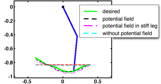
Fig. 7. Foot trajectory during stance phase for the three cases examined.
