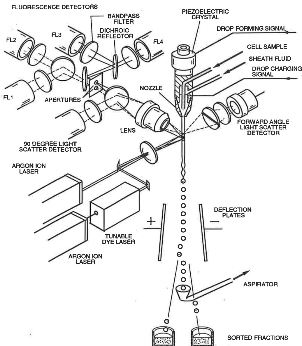
FIG. 1. Diagram of a typical two laser cell sorter (fluid, mechanical, and optical elements).
