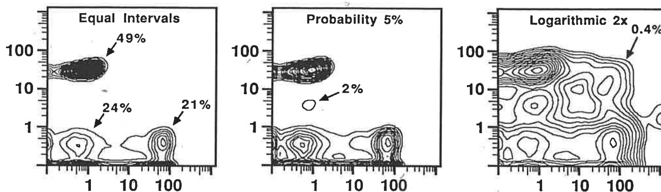
FIG. 5. Equal interval, probability, and logarithmic contour displays of a single set of two-color immunofluorescence data. The cell sample was a human peripheral blood lymphocyte preparation stained for CD8 (Leu-2a-Texas Red, horizontal axis ) and CD4 (Leu-3-phycoerythrin, vertical axis ). The three main subpopulations include 49% ( CD4^+ , CD8^- ), 24% ( CD4^- , CD8^- ), and 21% ( CD4^- , CD8^+ ) of the lymphocytes. The CD4 -low ^+ , CD8^- subpopulation seen in the logarithmic plot and marked by a single contour in the probability plot includes 2% of the lymphocytes, and the CD4^+ , CD8^+ subpopulation seen only in the logarithmic plot includes 0.4%.
