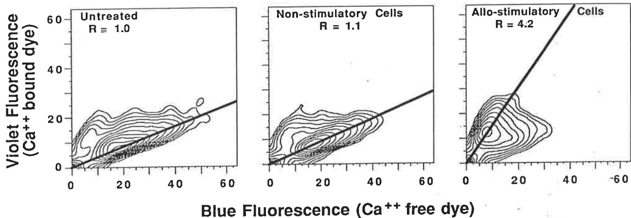
FIG. 12. Response of an Indo-1-labeled alloreactive T cell clone to appropriate and inappropriate "stimulator" cells. Indo-1 fluorescence is predominantly blue in the absence of \text{Ca}^{2+} and shifts to the violet when \text{Ca}^{2+} is bound. The violet/blue ratio ( R , defined here to be 1.0 for the resting cells shown in the left panel ) is indicative of the \text{Ca}^{2+} concentration to which the dye is exposed with higher ratios corresponding to higher \text{Ca}^{2+} concentrations. Clone B10 cells proliferate when exposed to clone MAK cells but not when exposed to clone MAR cells. Bringing B10 and "stimulator" cells into contact by centrifugation has little effect when clone MAR is used ( middle panel ) but with clone MAK a large increase in free intracellular \text{Ca}^{2+} concentration is observed ( right panel ). This effect occurs on a time scale of minutes rather than the several days needed for a proliferation assay. The figure panels all show logarithmic contours at twofold intervals.
