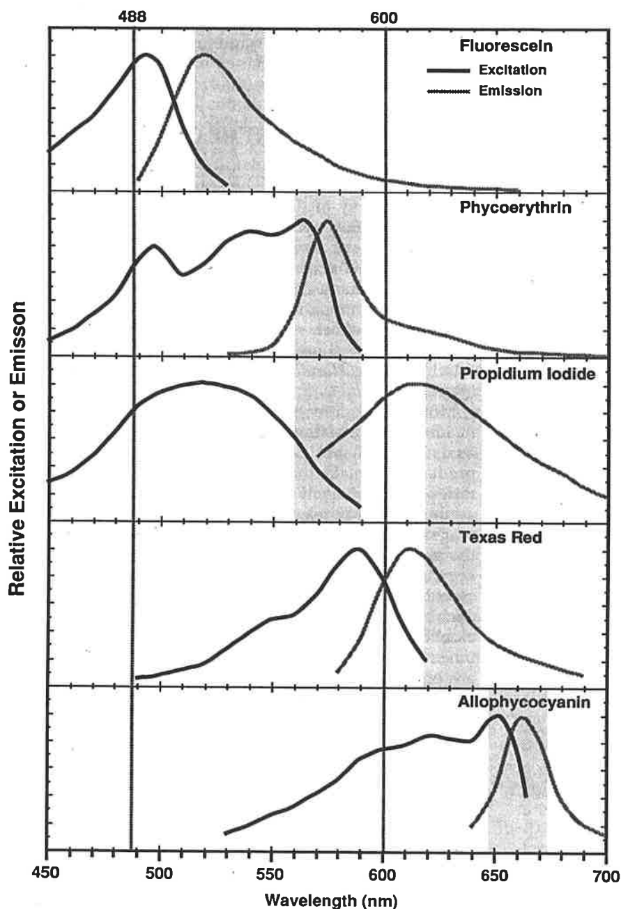
FIG. 2. Excitation and emission spectra of dyes commonly used for immunofluorescence in flow cytometry. The lines at 488 and 600 nm mark, respectively, typical argon ion laser and tunable dye laser wavelengths used for immunofluorescence excitation. The shaded bands indicate the detector acceptance ranges used to measure each dye. Propidium iodide fluorescence can be collected in either of the two marked regions.
