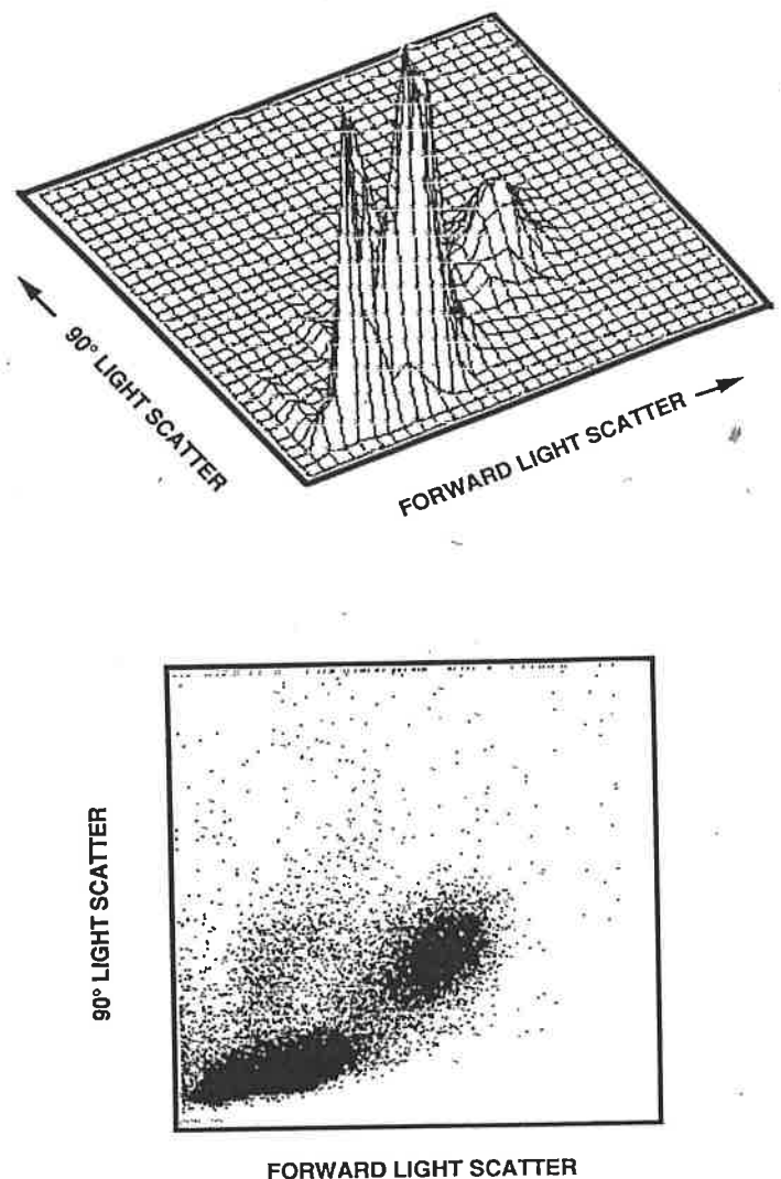
FIG. 4. Examples of two-parameter displays: a dot plot (lower panel) and a perspective plot (upper panel) of the same data. The measurements were forward light scatter and 90° light scatter on a "lymphocyte" preparation from human blood. From low light scatter to high light scatter the three major groups consist of dead cells, live lymphocytes, and live monocytes.
