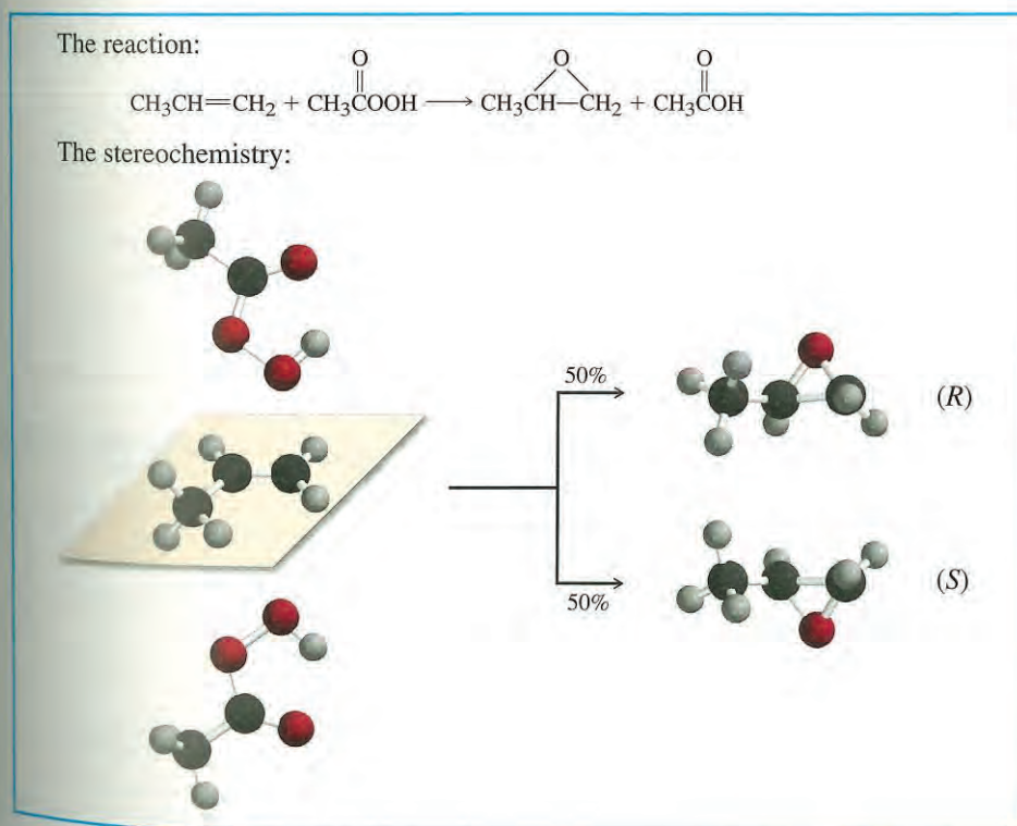
FIGURE 7.6 Epoxidation of propene produces equal amounts of ( R )- and ( S )-1,2-epoxypropane.
