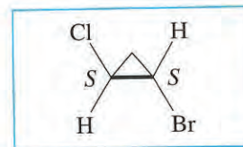
(1 S ,2 S )-1-Bromo-2-chlorocyclopropane
