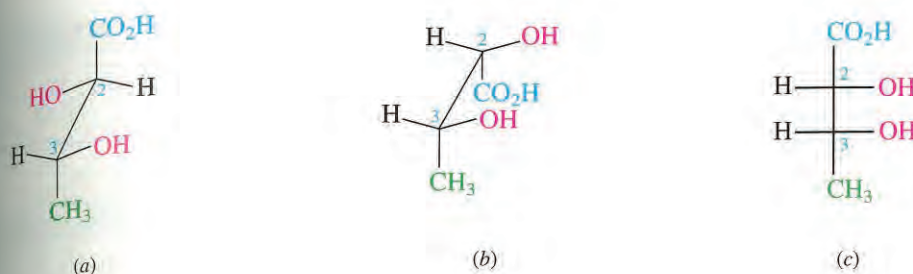
FIGURE 7.8 Representations of (2 R ,3 R )-dihydroxybutanoic acid. (a) The staggered conformation is the most stable, but is not properly arranged to show stereochemistry as a Fischer projection. (b) Rotation about the C-2–C-3 bond gives the eclipsed conformation, and projection of the eclipsed conformation onto the page gives (c) a correct Fischer projection.
