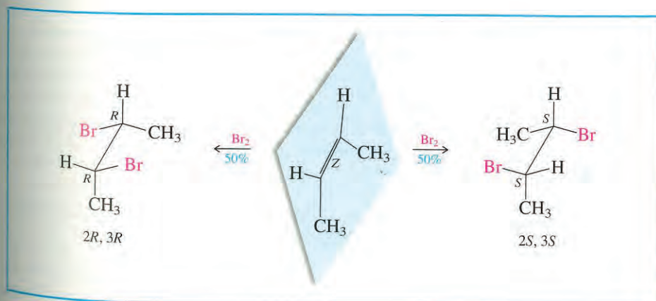
FIGURE 7.13 Anti addition of \text{Br}_2 to (Z) -2-butene gives a racemic mixture of (2R,3R) - and (2S,3S) -2,3-dibromobutane.
