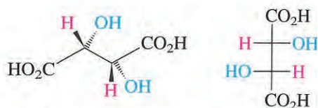
(2 R ,3 R )-Tartaric acid (mp 170°C, [\alpha]_D +12^\circ )
