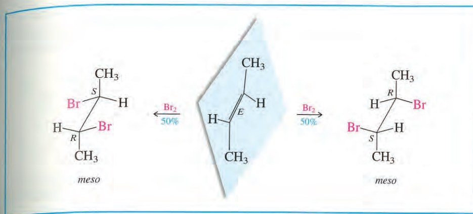
FIGURE 7.12 Anti addition of \text{Br}_2 to (E) -2-butene gives meso -2,3-dibromobutane.
