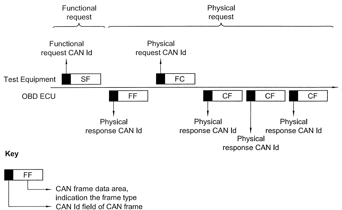
Figure 6 — CAN identifier usage
