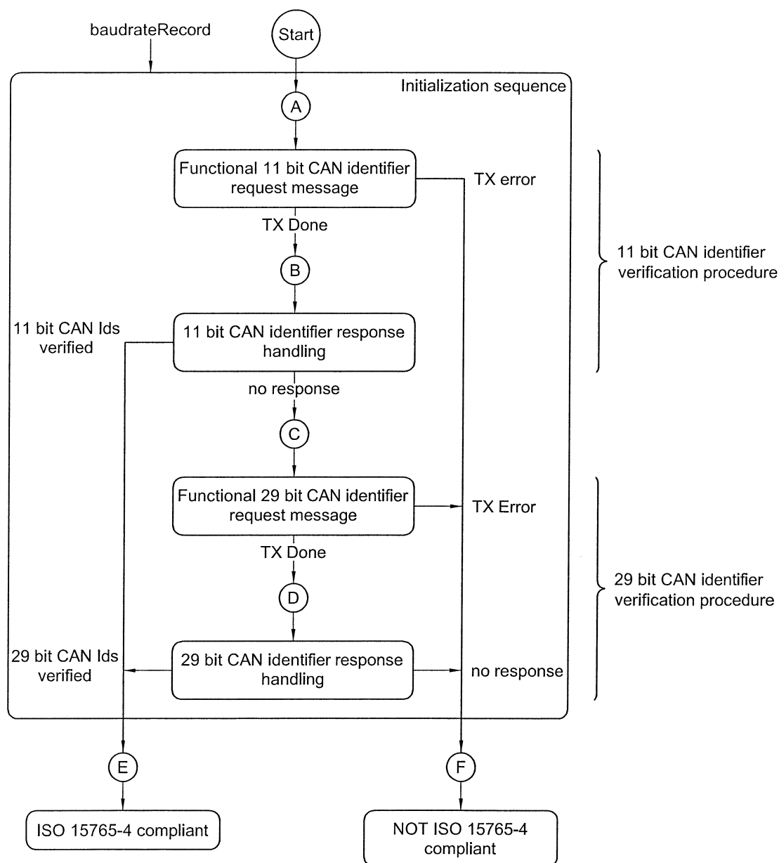
Figure 1 — Initialization sequence — Overview
