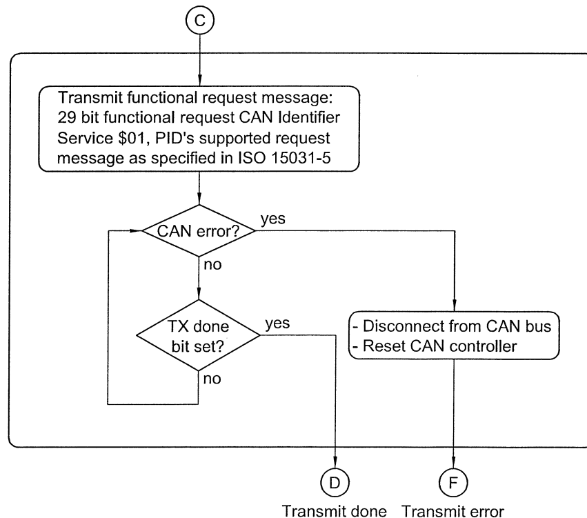
Figure 4 — Initialization sequence — 29 bit CAN identifier request transmission
