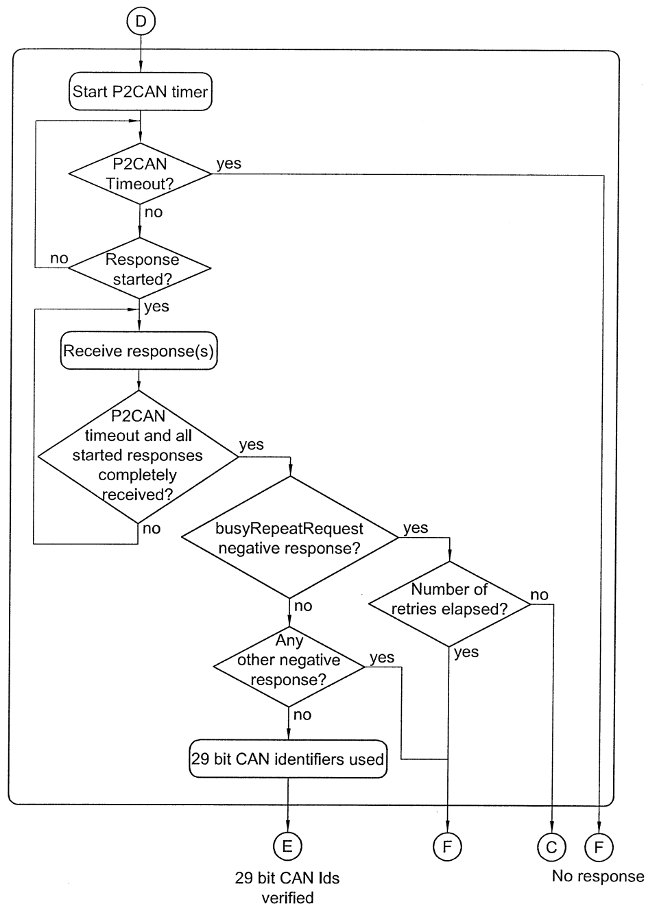
Figure 5 — Initialization sequence — 29 bit CAN identifier response handling
