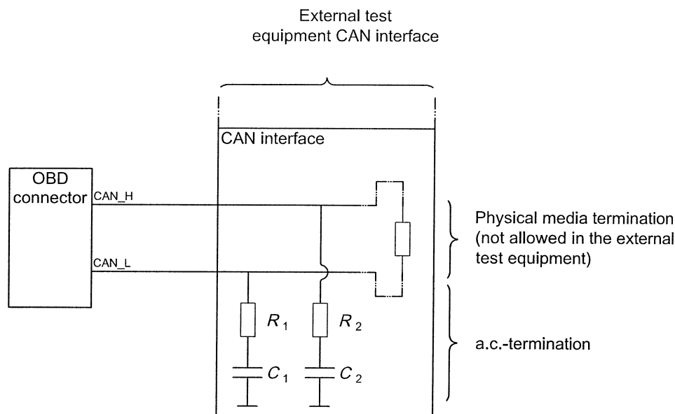
Figure 9 — External test equipment CAN bus termination
