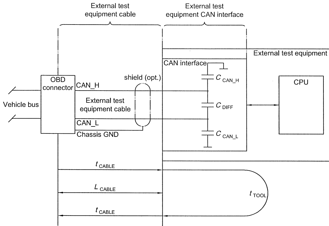
Figure 8 — External test equipment electrical parameters
