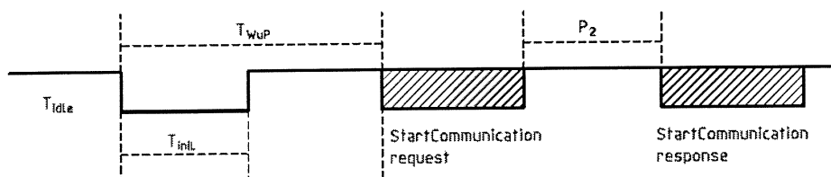
Figure 11 — Fast initialization
