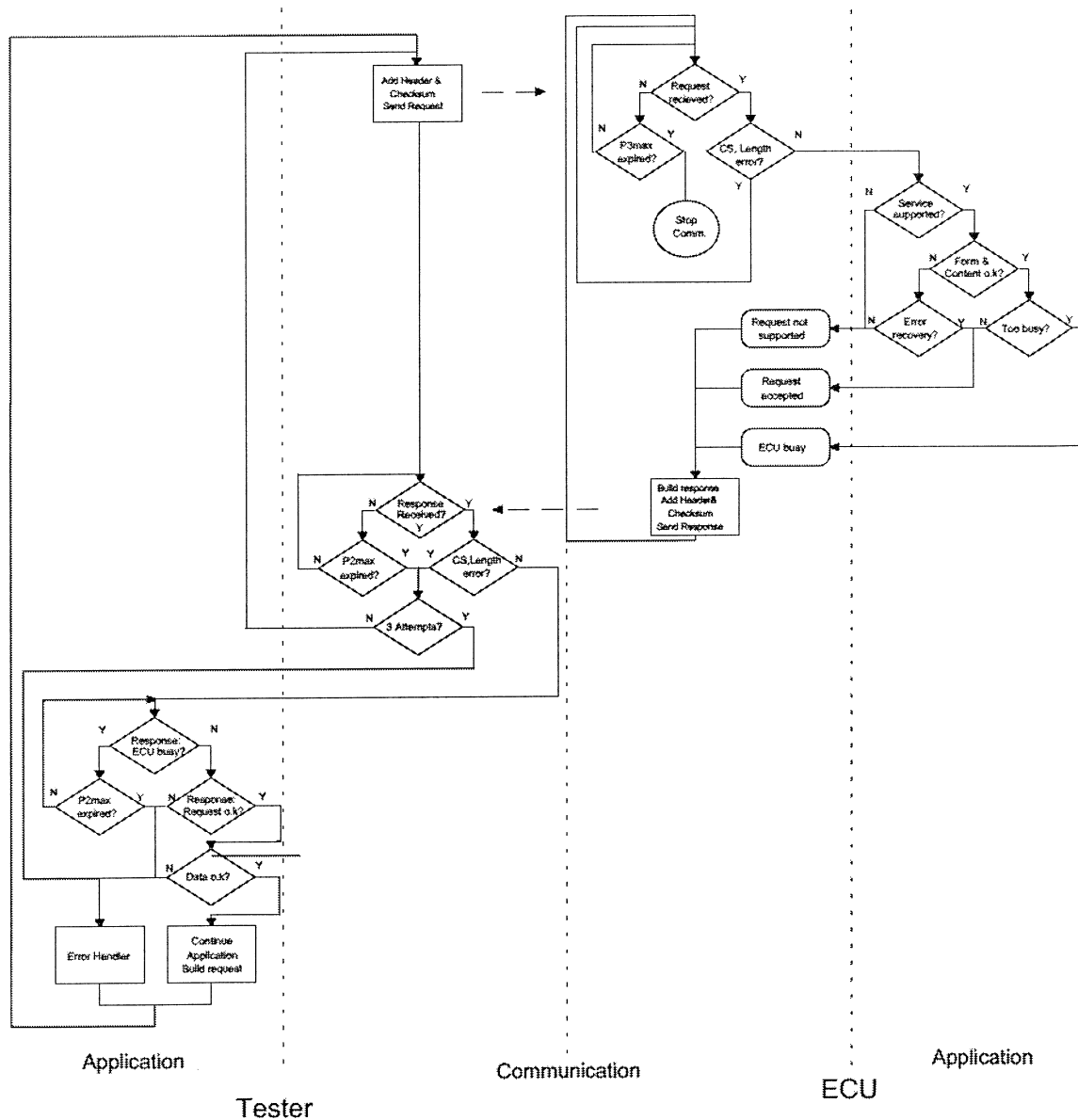
Figure 12 — Error handling
