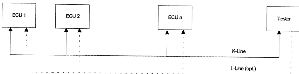
Figure 3 — Topology
