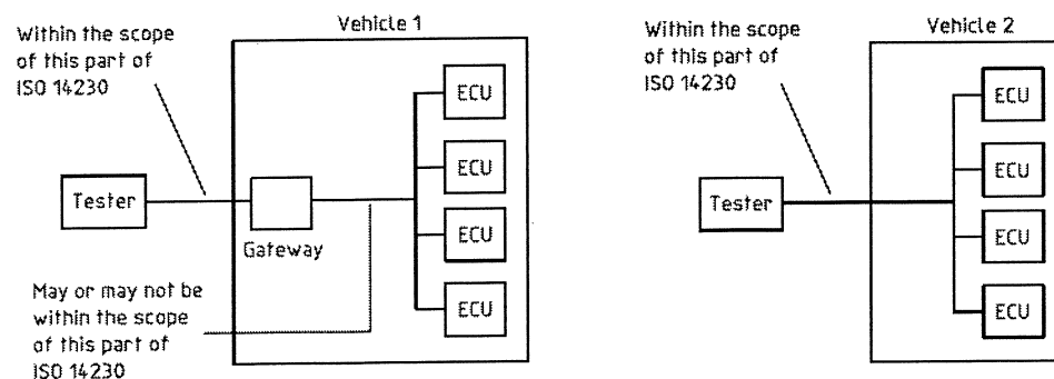
Figure 2 — Vehicle diagnostic architecture
