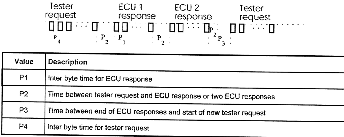
Figure 6 — Timing
