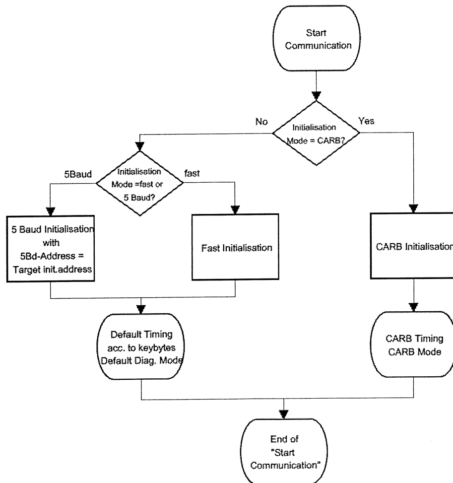
Figure 8 — Initialization modes
