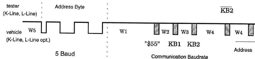
Figure 10 — 5 Baud initialization
