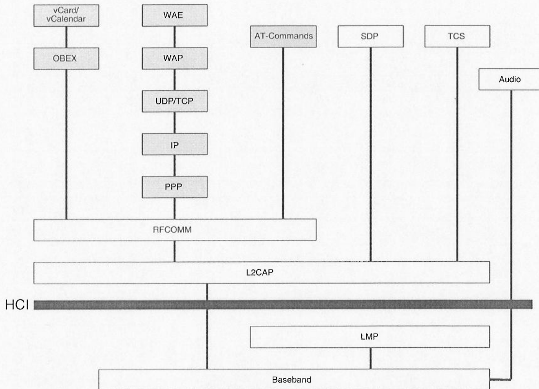
Figure 1. The Bluetooth Protocol Stack
