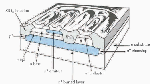
Fig. 7 Perspective view of an oxide-isolated bipolar transistor.
