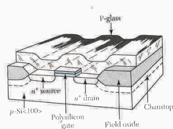
Fig. 15 Perspective view of an n -channel MOSFET. 7
