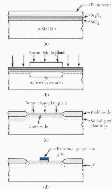
Fig. 16 Cross-sectional view of NMOS fabrication sequence. 7 (a) Formation of \text{SiO}_2 , \text{Si}_3\text{N}_4 , and photoresist layer. (b) Boron implant. (c) Field oxide. (d) Gate.
