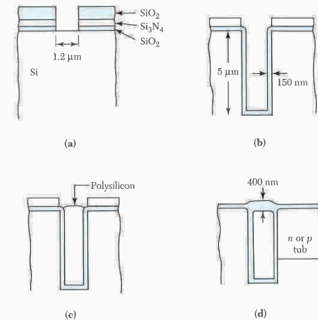
Fig. 26 Process sequence for forming a deep, narrow-trench isolation structure. (a) Trench mask patterning. (b) Trench etching and oxide growth. (c) Polysilicon deposition to fill the trench. (d) planarization.
