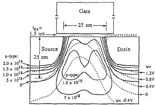
Fig. 5-29 Doping contours in 25-nm PMOSFET. 53
