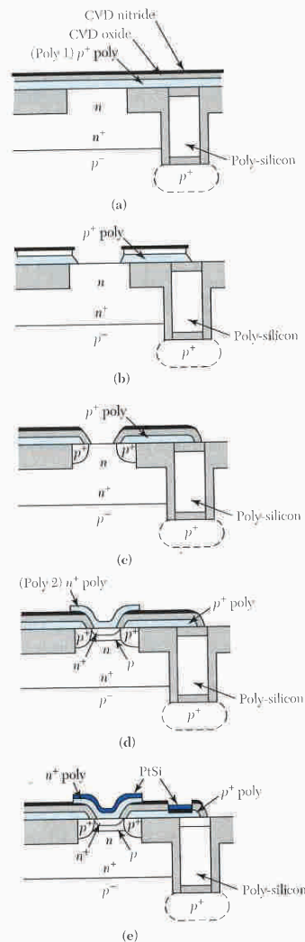
Fig. 13 Process sequence for fabricating double-polysilicon self-aligned n - p - n transistors. 6f
