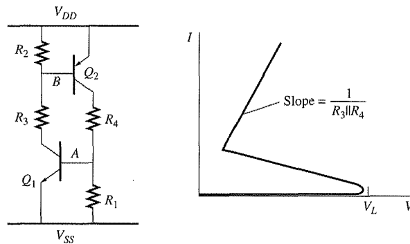
(b) IV characteristic of pnp – npn structure
