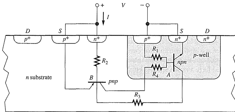
(a) Origin of parasitic elements
