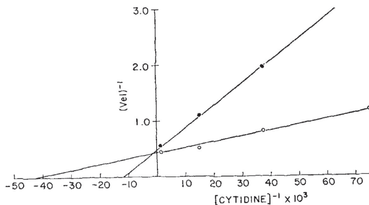
FIG. 3. Competitive inhibition of the deamination of cytidine by 5-azacytidine, 6.7 \times 10^{-4} \text{ M} . Cytidine- 2\text{-}^{14}\text{C} was incubated with enzyme in the presence of unlabeled 5-azacytidine, and uridine- 2\text{-}^{14}\text{C} was isolated as described in text. (○—○) = cytidine- 2\text{-}^{14}\text{C} ; (●—●) = cytidine- 2\text{-}^{14}\text{C} with 5-azacytidine.
