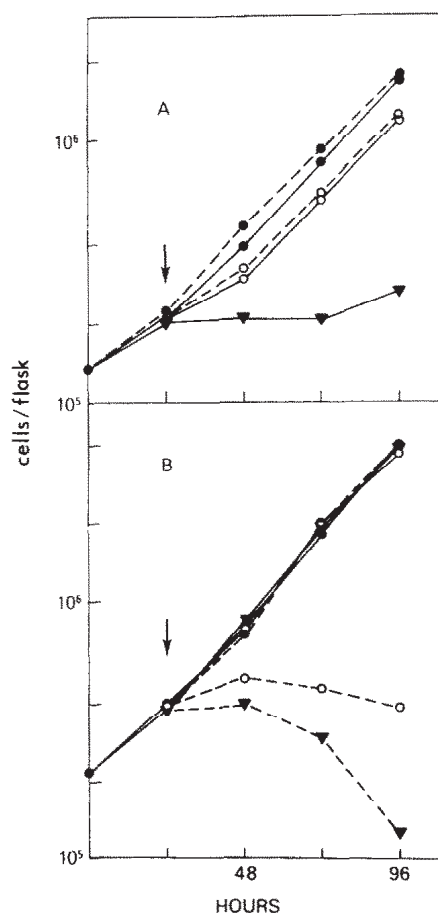
Fig. 1. Growth of HeLa cells in the presence of azaC, DHazaC and THU. (a) ●—●, control; ●—●, 100 \mu\text{M} THU; ○—○, 1 \mu\text{M} azaC; ○—○, 1 \mu\text{M} azaC plus 100 \mu\text{M} THU; ▼, 10 \mu\text{M} azaC. (b) ●—●, control; ●—●, 100 \mu\text{M} THU; ○—○, 100 \mu\text{M} DHazaC; ○—○, 100 \mu\text{M} DHazaC plus 100 \mu\text{M} THU; ▼, 200 \mu\text{M} DHazaC; ▼—▼, 200 \mu\text{M} DHazaC plus 100 \mu\text{M} THU. Arrows indicate when drugs were administered.
