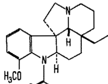
(–)-Aspidospermin (VII)
