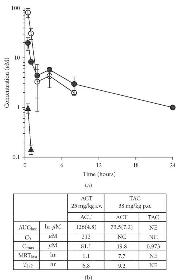
FIGURE 2: Pharmacokinetics of oral TAC versus i.v. 5-azacitidine in C57BL/6 mice. (a) Mean plasma concentration versus time for triacetyl azacitidine (TAC) ( \blacktriangle ) and resultant ACT ( \bullet ) in nontumor bearing mice after a 38 mg/kg dose of oral TAC. Mean plasma concentration versus time for ACT in nontumor bearing mice after 25 mg/kg ACT i.v. ( \circ ). Error bars indicate standard deviation. (b) Noncompartmental plasma pharmacokinetic parameters for azacitidine (ACT) and tri-acetyl azacitidine (TAC). \text{AUC}_{\text{last}} values are mean (standard error). NE—not estimated. NC—not calculated.
