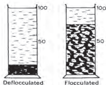
Fig 19-33. Sedimentation parameters of suspensions. Deflocculated suspension: F_\infty = 0.15 . Flocculated suspension: F = 0.75 ; \beta = 5.0 .
