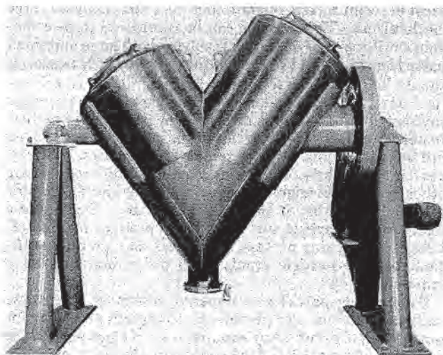
Fig 88-21. Cross-Flow twin-shell blender (courtesy, Patterson-Kelley).
