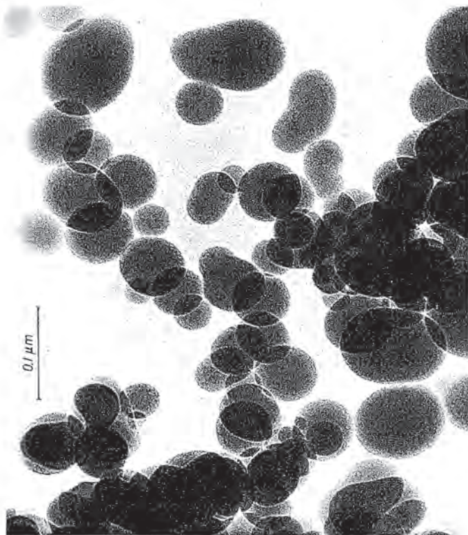
Fig 19-26. Transmission electron micrograph of Aerosil OX 50, ground and dusted on. The spheres are translucent to the electron beam, causing overlapping portions to be darker owing to increased thickness (courtesy, Degussa AG of Hanau, West Germany; Aerosil is a registered trademark of Degussa). The suffix 50 indicates the specific surface area in m 2 /g.
