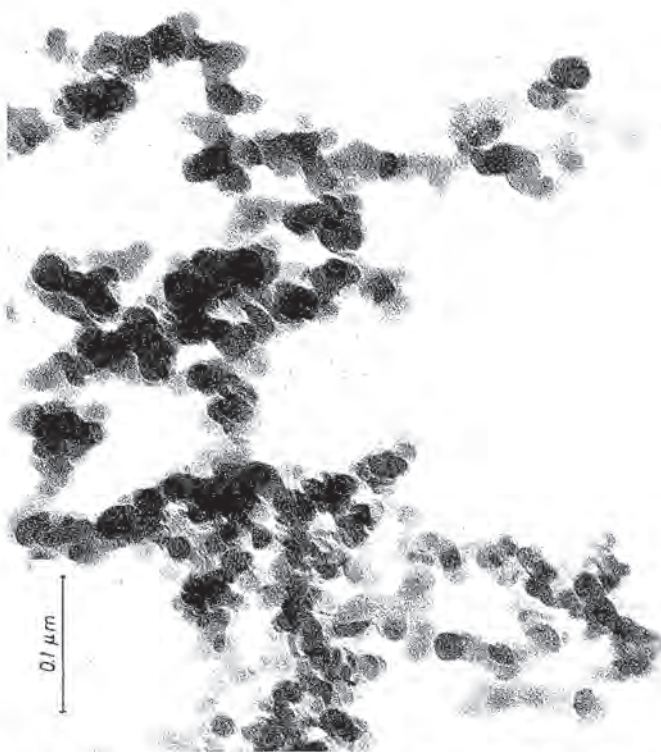
Fig 19-27. Transmission electron micrograph of Aerosil 130, ground and dusted on. The spheres are fused together into chain-like aggregates (courtesy, Degussa AG of Hanau, West Germany; Aerosil is a registered trademark of Degussa). The suffix 130 gives the specific surface area in m 2 /g.
