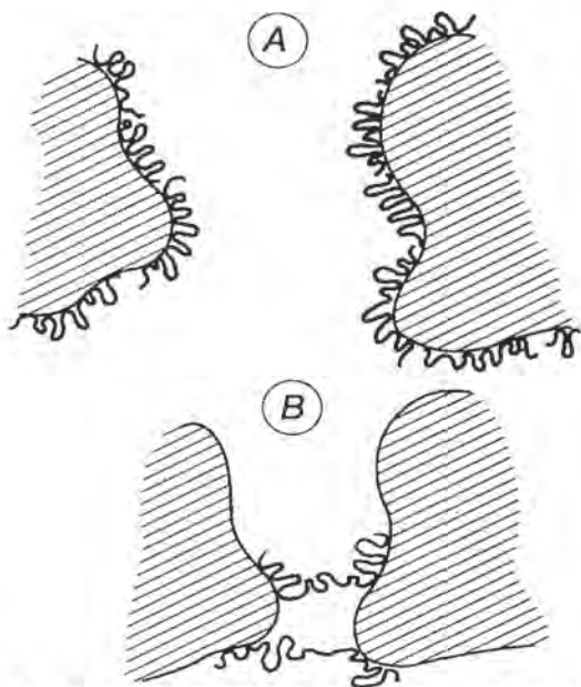
Fig 19-31. Protective action (A) and sensitization (B) of sols of hydrophobic particles by adsorbed polymer chains.
