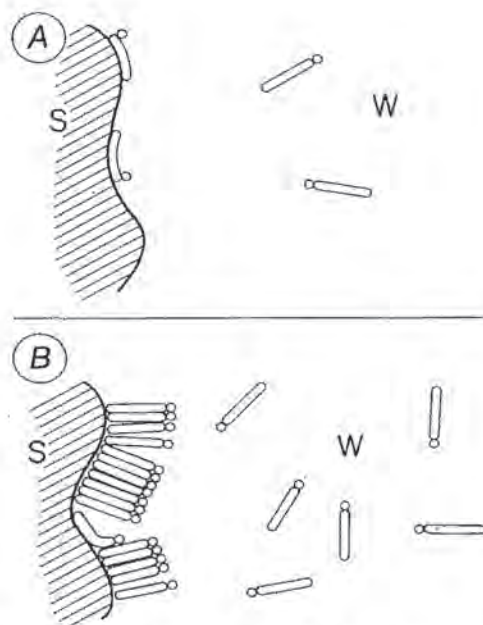
Fig 19-30. Schematic representation of the physical adsorption of surfactant molecules at a hydrophobic solid (S)/water (W) interface. Cylindrical portions and spheres represent hydrocarbon chains and polar headgroups of the surfactant molecules, respectively. (A) low surfactant concentration/low surface coverage; (B) near critical micelle concentration/surface coverage near saturation.
