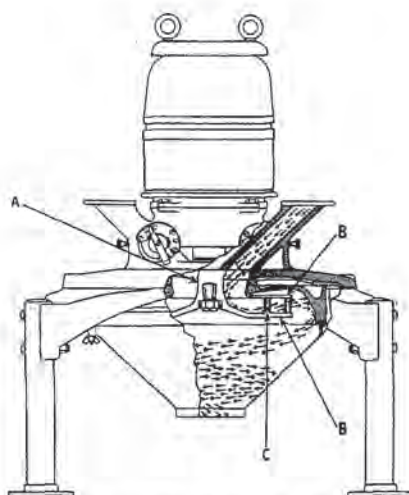
Fig 88-6. CentriMil, a centrifugal-impact mill, available in models ranging from 2 to 250 hp. A: Spinning rotor; B: rotor hub disks; C: impactors (courtesy, Entoletter).
