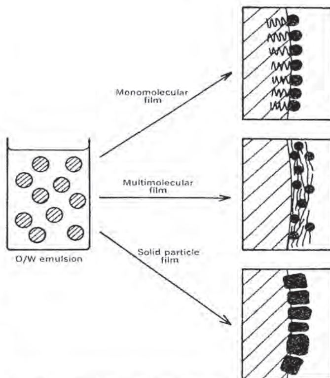
Fig 19-37. Types of films formed by emulsifying agents at the oil/water interface. Orientations are shown for O/W emulsions. ▨: oil; □: water.
