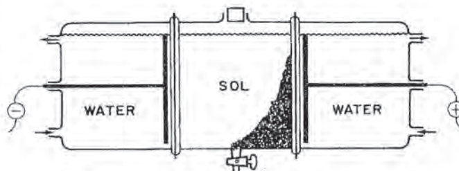
Fig 19-21. Electrodialyzer showing electrodecentration.
