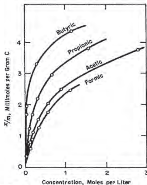
Fig 19-15. The relation between adsorption and molecular weight of fatty acids. 9
