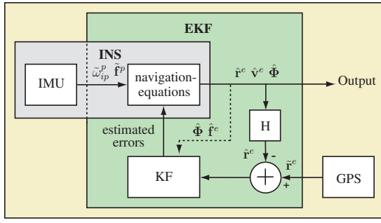
Fig. 4. The INS provides the main navigation solution. When GPS data is available the position error is estimated and used as the input to a Kalman filter, estimating the navigation errors. The errors are fed back to the INS for correction of internal states.
