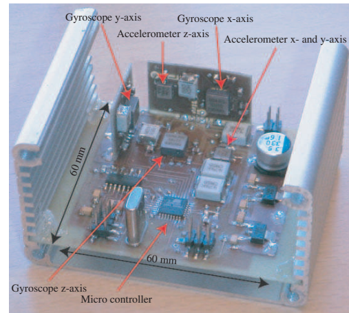
Fig. 3. The inhouse constructed inertial measurement unit. In the upper part of the picture the three gyros and the double axed and single axed accelerometer can be seen. In the lower part of the picture the micro-controller can be seen, responsible for sampling of the sensors. Altogether the IMU measures 60 \times 60 \times 25 mm.
