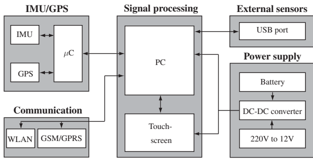
Fig. 2. Block-diagram of the navigation platform. The platform is constructed around five modules.
