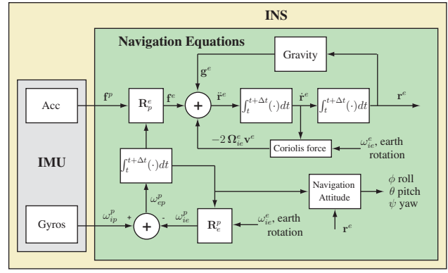
Fig. 5. The block diagram corresponds to ECEF navigation equations used in the INS.
