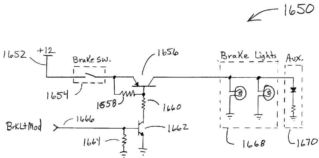
FIG. 35 Brake Light Modulation Circuit
