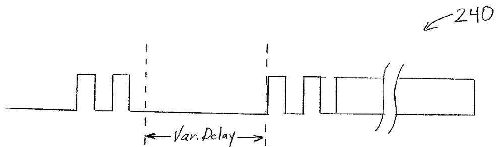
FIG. 7 Packet Header
