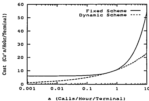
Figure 1: Normalized bandwidth cost vs. a
