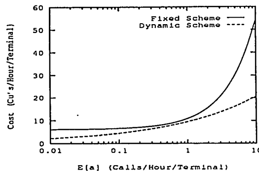
Figure 5: Normalized cost as function of \bar{a}
