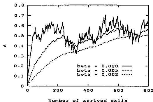
Figure 3: Variations of A with different \beta
