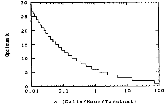
Figure 2: k_{opt} as function of a
