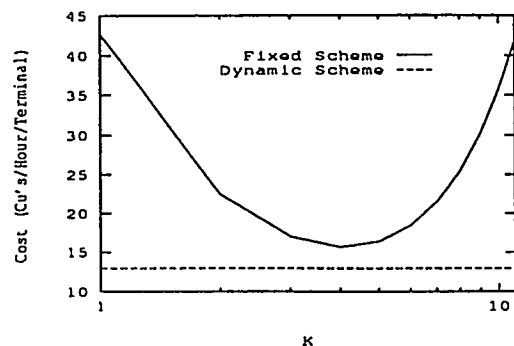
Figure 4: Normalized cost as function of k
