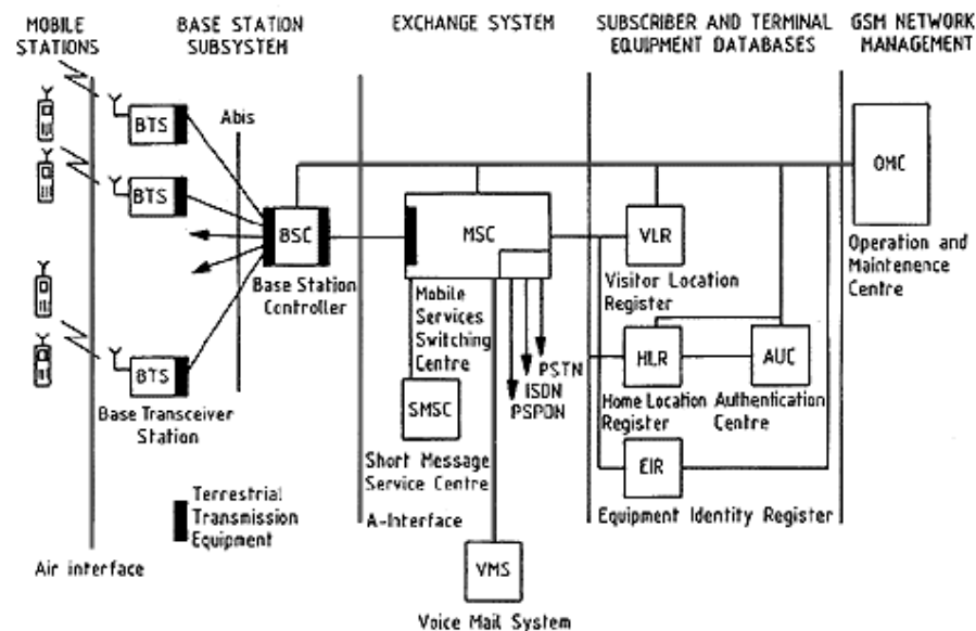
Fig 1. GSM network architecture
