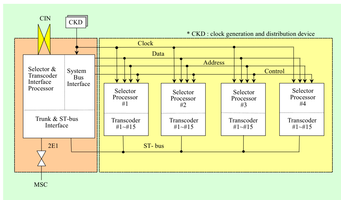
Fig. 7. TSB structure.
