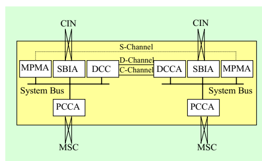
Fig. 10. CCP structure.
