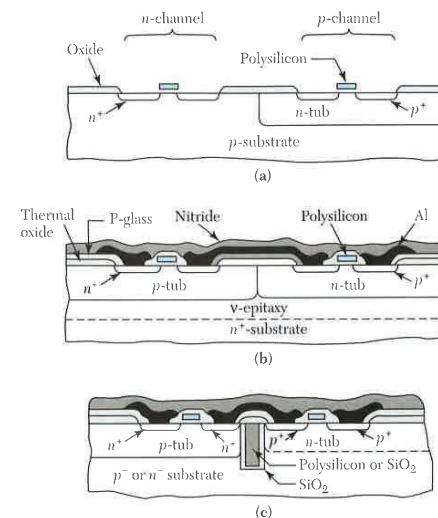
Fig. 24 Various CMOS structures. (a) n -tub. (b) Twin tub 4 . (c) Refilled trench. 11
