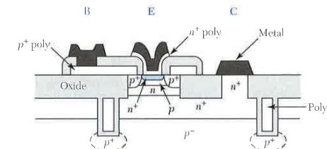
Fig. 12 Cross-section of a self-aligned, double-polysilicon bipolar transistor with advanced trench isolation. 5
