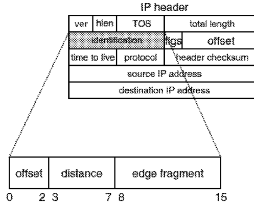
Figure 9: Encoding edge fragments into the IP identification field.
