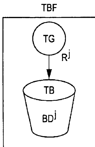
COMPONENTS OF A TOKEN BUCKET FILTER
