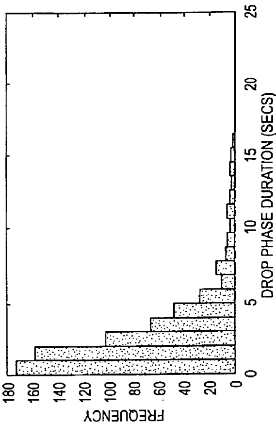
NON-DCM SCHEME AT UTILIZATION = 0.9
