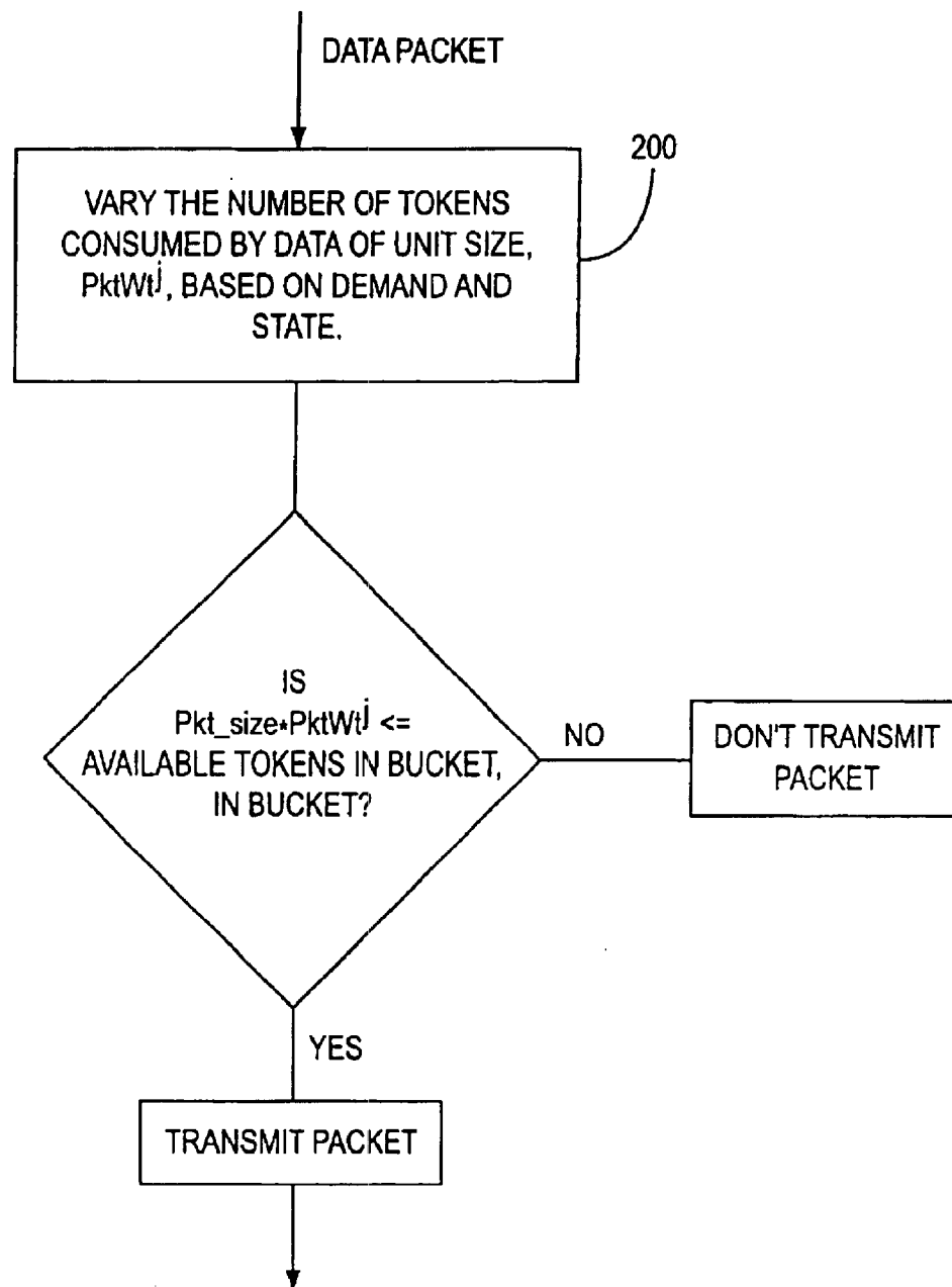
FLOWCHART FOR TBF-BASED RATE CONTROL METHOD
