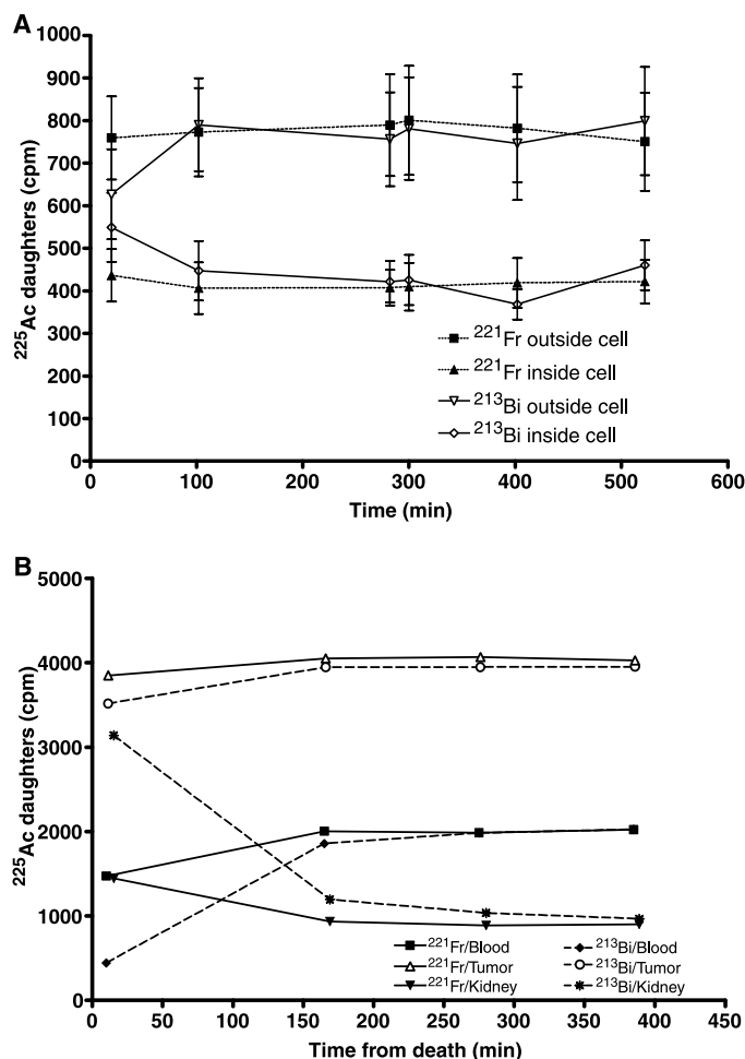
Fig. 1. (A) Internalization and retention in vitro of ^{225}\text{Ac} ]J591/ ^{213}\text{Bi} / ^{221}\text{Fr} in LNCaP cells. Actinium-225 that was internalized or was outside the cell was determined after a 5-hour period when secular equilibrium was established and the ^{213}\text{Bi} and ^{221}\text{Fr} curves converge. The radionuclidic decay of ^{225}\text{Ac} yields two daughter radionuclides, ^{221}\text{Fr} and ^{213}\text{Bi} , that can be monitored in these experiments by gamma spectroscopy. Values shown are mean \pm SD. LNCaP cells ( 10^7 cells) were exposed to an antibody-to-antigen excess of ^{225}\text{Ac} ]J591 at 37°C for 90 min [supplementary note 3 (11)]. (B) Biodistribution in vivo of ^{225}\text{Ac} ]J591/ ^{213}\text{Bi} / ^{221}\text{Fr} in several tissues from one representative mouse. Actinium-225 that was tissue-associated was determined after a 5-hour period when secular equilibrium was established and the ^{213}\text{Bi} and ^{221}\text{Fr} curves converge. Pharmacological analysis of the two ^{225}\text{Ac} daughters was performed in vivo by injecting 12 kBq of ^{225}\text{Ac} ]J591 or 12 kBq of ^{225}\text{Ac} ]HuM195 (irrelevant control) intraperitoneally in two groups of male athymic nude mice ( n = 12 per group) (Taconic, Germantown, New York) bearing a 3- to 4-week-old LNCaP i.m. tumor xenograft. Mice from each group were killed at days 2 and 3, respectively, and the tumors, blood, and other tissues were removed and immediately counted with a Packard Cobra Gamma Counter using two energy windows [supplementary note 3 (11)].
