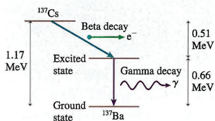
FIGURE 42.23 The decay of ^{137}\text{Cs} involves both beta and gamma decay.
