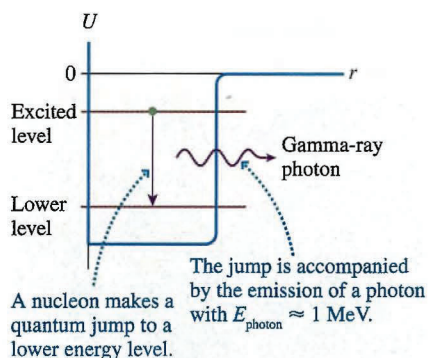
FIGURE 42.22 Gamma decay.
