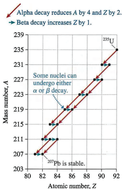
FIGURE 42.24 The nuclear decay series of ^{235}\text{U} .
