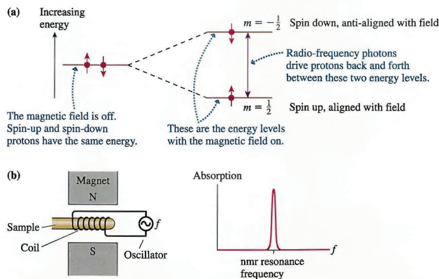
FIGURE 42.26 Nuclear magnetic resonance is possible because spin-up and spin-down protons have slightly different energies in a magnetic field.
