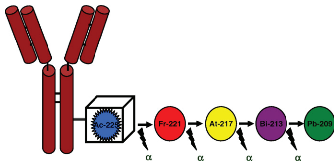
Fig. 2. An illustration of the ^{225}\text{Ac} nanogenerator system.
