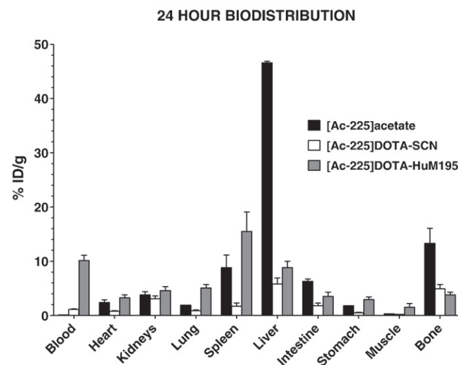
Fig. 3. Murine biodistribution data at 24 h for ^{225}\text{Ac} -acetate, [ ^{225}\text{Ac} ]DOTA-SCN, and [ ^{225}\text{Ac} ]DOTA-HuM195.
