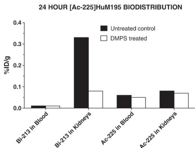
Fig. 4. Biodistribution data at 24 h for [ ^{225}\text{Ac} ]DOTA-HuM195 administered to two cynomolgus monkeys. Note the reduction in the renal ^{213}\text{Bi} activity in the DMPS-treated monkey as compared to an untreated (no DMPS) animal.
