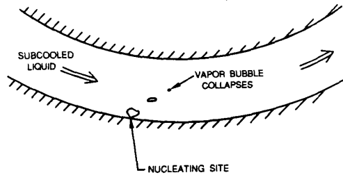
Figure 6 Bubble Generation and Collapse During Subcooled Boiling in a Curved Channel.
