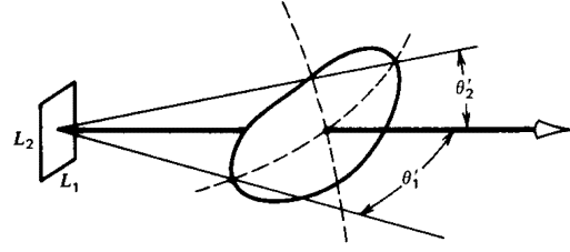
Figure 7.6.4 Area of the unit sphere ensonified by a plane piston source of arbitrary shape.
