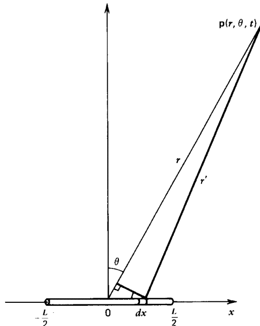
Figure 7.3.1 The far field acoustic field at (r, \theta) of a continuous line source of length L and radius a is found by summing the contributions of simple sources of length dx and radius a .
