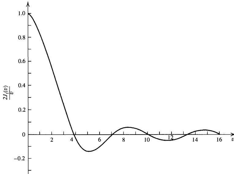
Figure 7.4.4 Functional behavior of 2J_1(v)/v .
