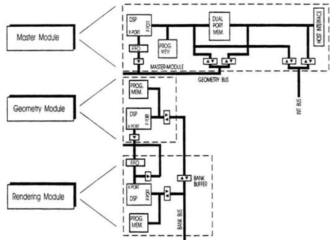
FIGURE 4.2. Basic module structure
