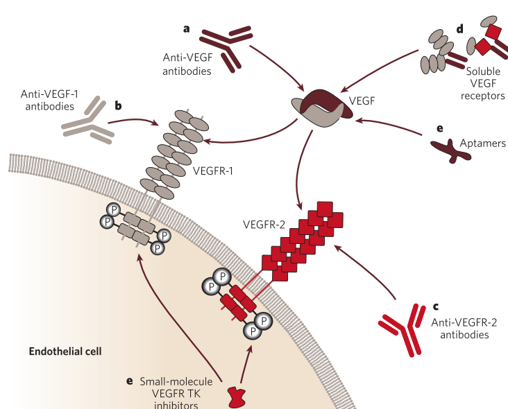
Figure 3 | Various strategies to inhibit VEGF signalling. These include monoclonal antibodies targeting VEGF-A (a) or the VEGF receptors (b, c). d, Chimeric soluble receptors such as the 'VEGF-trap' (domain 2 of VEGFR-1 and domain 3 of VEGFR-2 fused to a Fc fragment of an antibody) are also undergoing clinical development. e, Additional extracellular inhibitors are aptamers that bind the heparin-binding domain of VEGF165 (pegaptanib). A variety of small-molecule VEGF RTK inhibitors that inhibit ligand-dependent receptor autophosphorylation of VEGFR-1 and VEGFR-2 are being tested. Additional strategies to inhibit VEGF signalling include antisense and siRNA targeting VEGF-A or its receptors.
