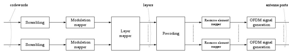
Figure 6.3-1: Overview of physical channel processing.
