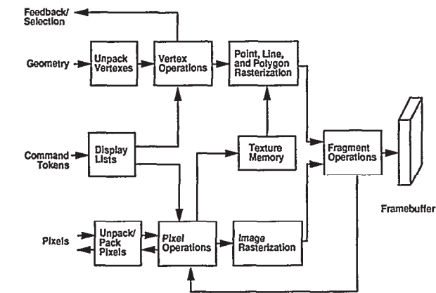
Figure 1: The dataflow within the OpenGL architecture’s conceptual state machine.
