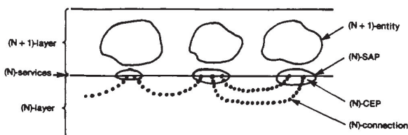
Fig. 5. Connections and connection endpoints (CEP's).
