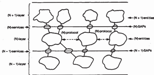
Fig. 4. Entities, service access points (SAP's), and protocols.
