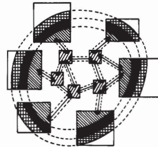
Fig. 2. Network layering.
