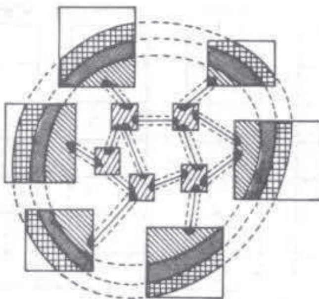
Fig. 2. Network layering.
