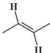
Figure 2. trans Double Bond
