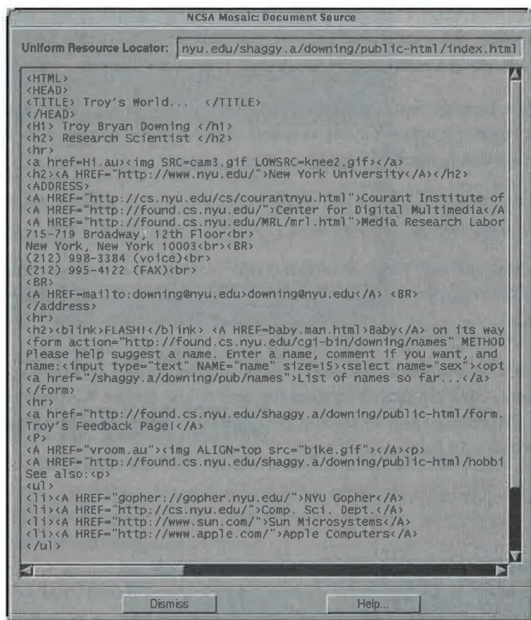
Figure 5-6 Peeking behind the scenes to see the source HTML markup of the current Web page
