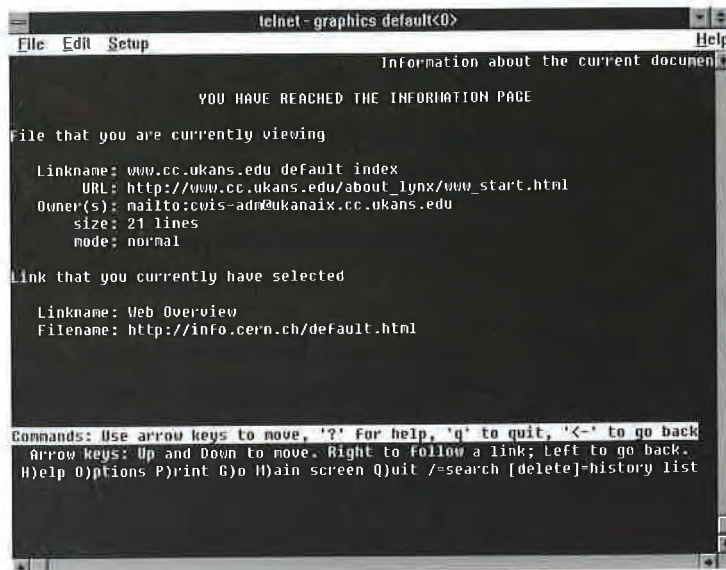
Figure 3-2 A screenful of information about the current Web page and the currently selected link
