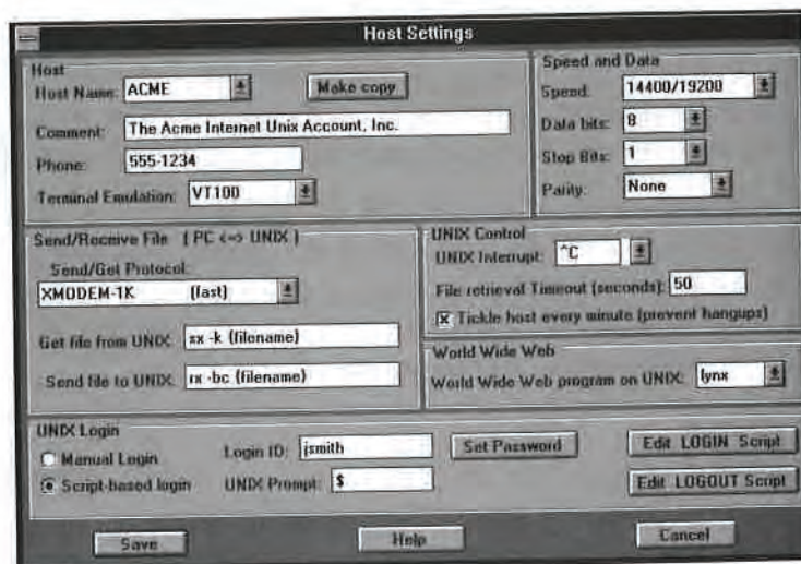
Figure 4-1 Everything SlipKnot needs to know about your host machine and isn't afraid to ask
