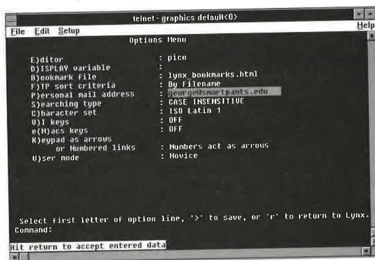
Figure 3-10 The Lynx Options Menu
