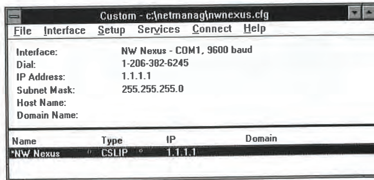
Figure I-3 Your customized on-ramp onto the Information Superhighway
