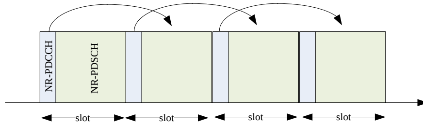
Figure 5: Cross-slot beam indication
