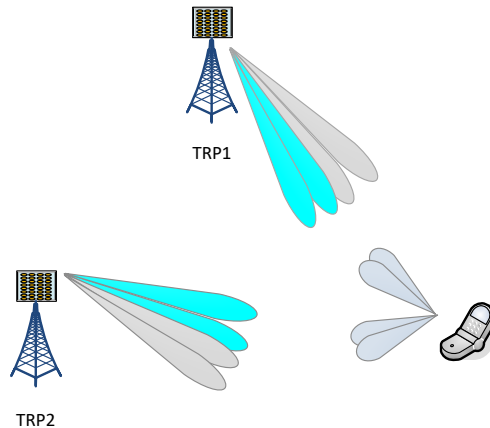
Figure 3: Illustration of group based beam reporting
