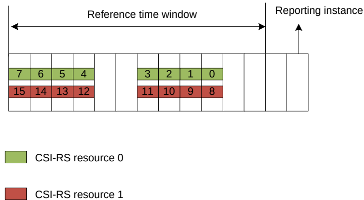
Figure 2: Reference time window configuration for indication of DL Tx beam
