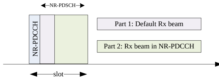
Figure 6: Beam indication based on partition of NR-PDSCH
