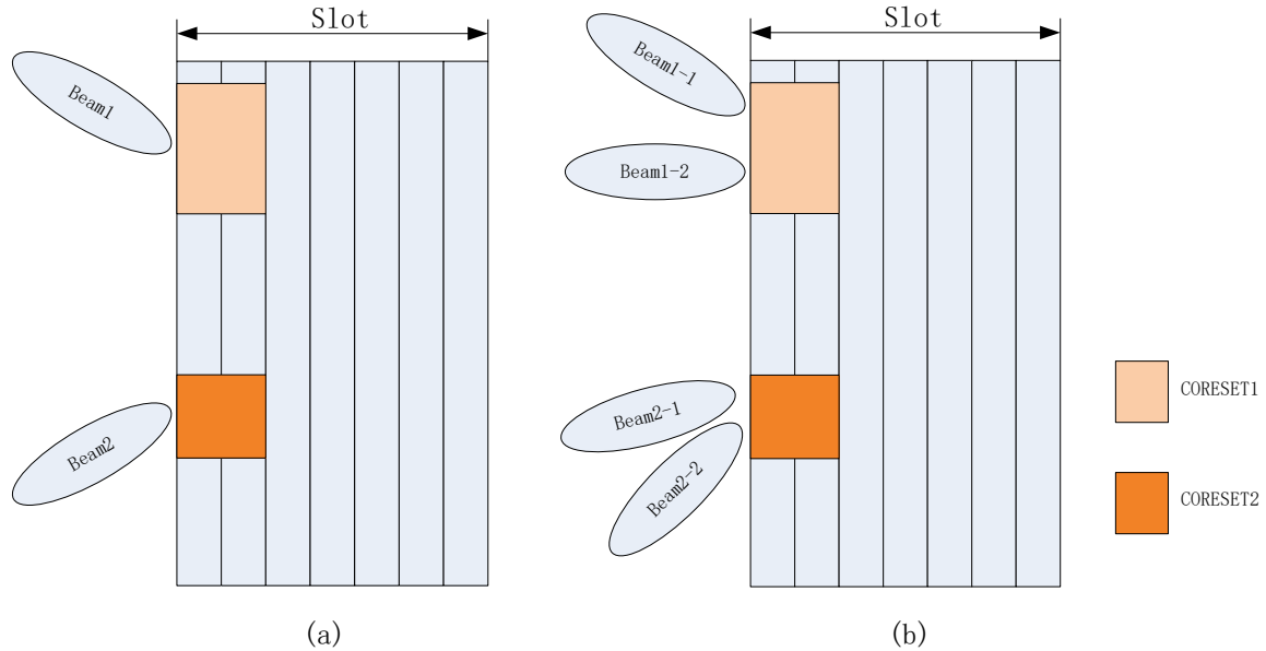
Figure4: Beam operation for UE-specific NR-PDCCH
