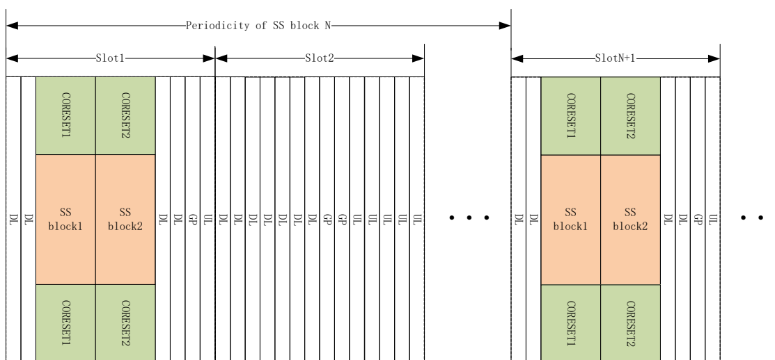
Figure2: First CORESET linked to SS-block
