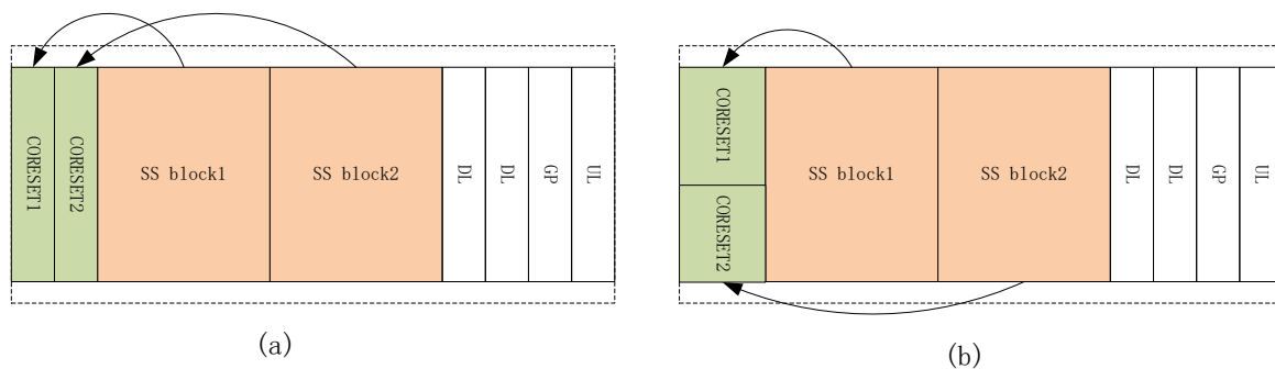
Figure3: First CORESET configured by MIB
