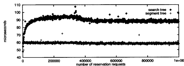
Figure 8: Admission decision speed within the LTU domain
