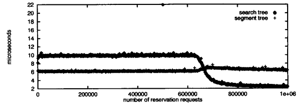
Figure 4: Admission decision speed for a single link
