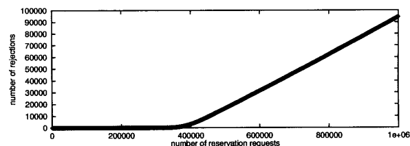
Figure 9: Admission rejections within the LTU domain
