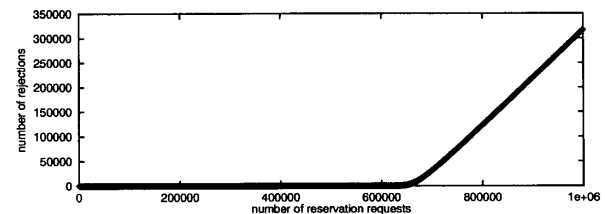
Figure 5: Rejections for a single link
