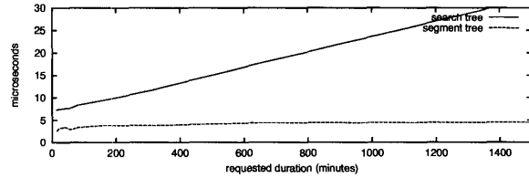
Figure 7: Decision time and length of requested durations
