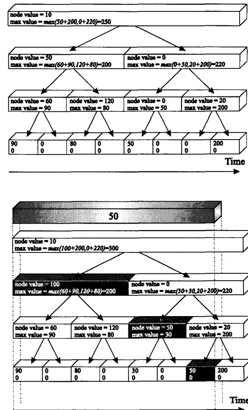
Figure 3: A segment tree before and after insertion
