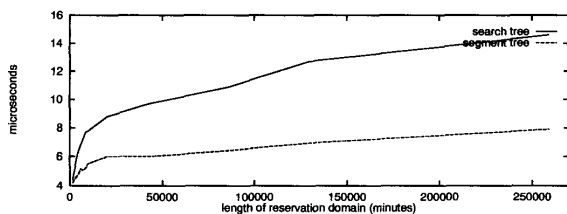
Figure 6: Decision time and reservable time frame
