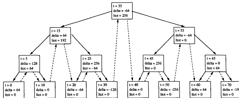
Figure 2: A binary search tree over time
