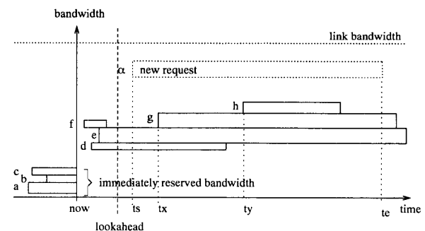
Figure 1: Advance reservations in a time-bandwidth domain
