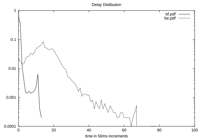
Figure 9: Delay distribution for best effort and EF UDP traffic
