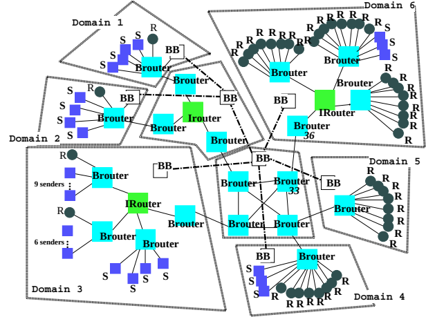
Figure 5: Simulation Topology
