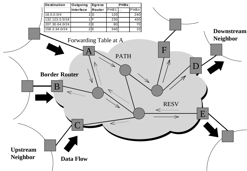
Figure 8: RSVP as intra-domain protocol
