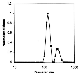
Figure 8. Dynamic light scattering analysis of lot B SFP.
