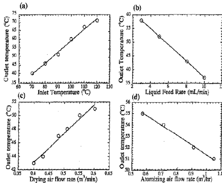
Figure 2. Measured dependencies of T_{outlet} in the Büchi laboratory spray-dryer on (a) T_{inlet} ; (b) v_L ; (c) v_{da} ; (d) v_{sa} . Standard spray-drying conditions used were: T_{inlet} = 90^\circ\text{C} , v_L = 5\text{ mL/min} , v_{da} = 900\text{ L/h} , v_{sa} = 600\text{ L/min} . Figure reproduced from Maa et al. (1997), with permission.
