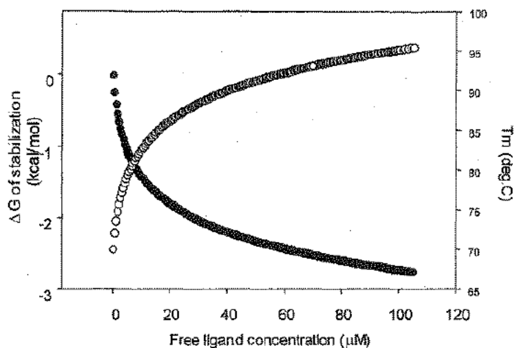
Figure 1. Hypothetical free energy of stabilization (filled circles) and corresponding increase in T_m (open circles) due to ligand binding to the native state ( K_a = 10^6 \text{ M}^{-1} ).
