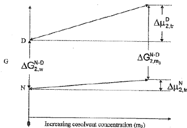
Figure 2.3. Free energy of N to D transition in the absence and presence of an excluded cosolvent.
