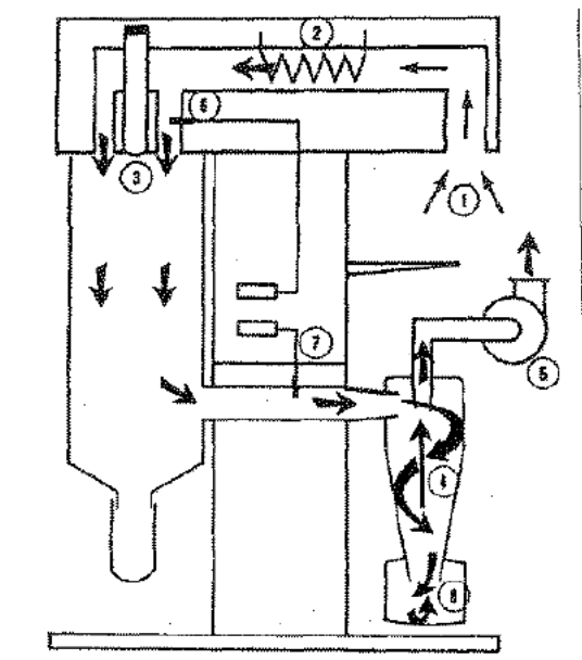
Figure 1. Schematic of Büchi laboratory spray dryer. (1) air inlet; (2) inlet-air heating element; (3) two-fluid nozzle; (4) cyclone separator; (5) ventilator fan; (6) thermocouple to measure T_{inlet} ; (7) thermocouple to measure T_{outlet} ; (8) product collector. Reproduced with permission of the manufacturer.
