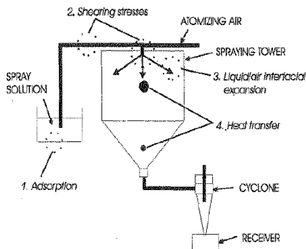
Figure 6. Schematic representation of the possible stresses experienced by a protein during spray-drying. See text for explanations. The current state of knowledge indicates that protein adsorption at the large liquid/air interface created during atomizing of the spray solution is mainly responsible for the protein aggregation/inactivation measured on spray-drying ("process instability" of the protein).
