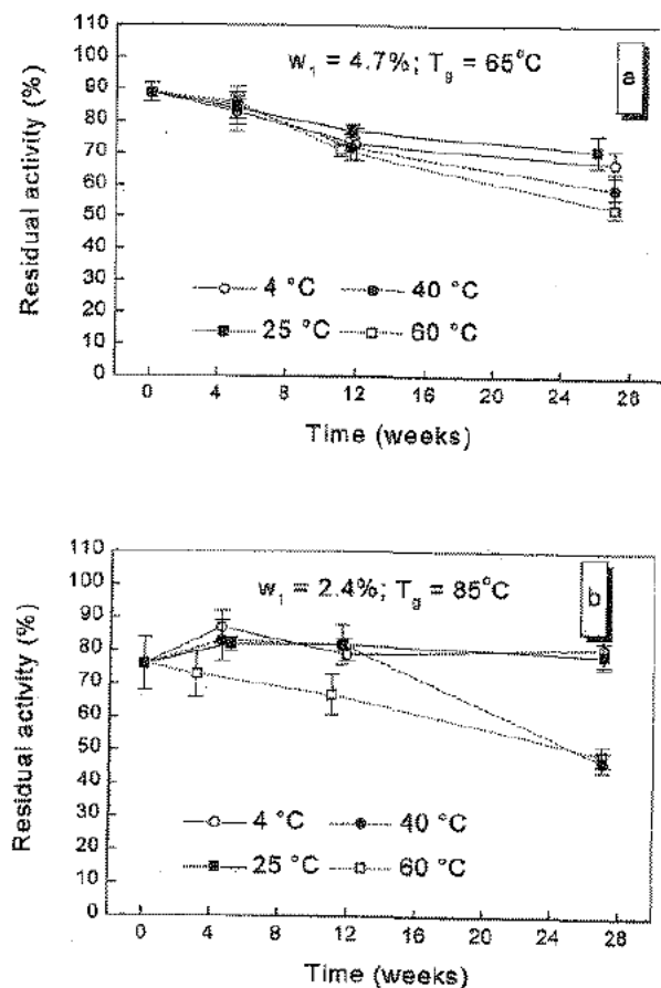
Figure 5. Residual activity of LDFI measured immediately after spray-drying at T_{\text{inlet}}/T_{\text{outlet}} = (a) 90^\circ\text{C}/60^\circ\text{C} , or (b) 150^\circ\text{C}/95^\circ\text{C} , and also on subsequent dry-storage at various temperatures. Reproduced from Adler and Lee (1999) with permission.
