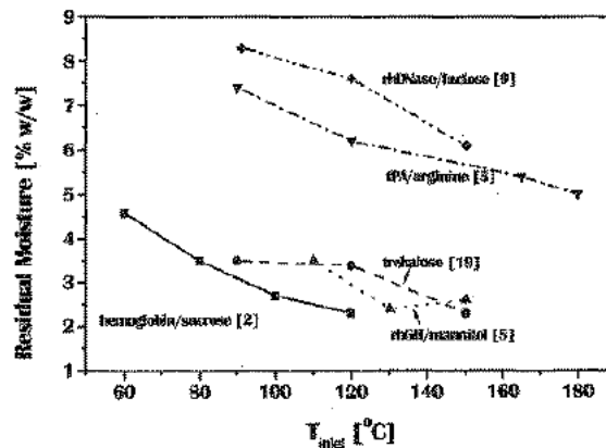
Figure 3. Relation between residual moisture and T_{inlet} for various spray-dried powders taken from the reference cited in the figure. The other independent process parameters ( v_{lf} , v_{at} & v_{da} ) were not in all cases the same in the various works. See text for explanations of the abbreviations used.
