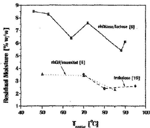
Figure 4. Relation between residual moisture and T_{outlet} for various spray-dried powders taken from the reference cited in the figure. The other independent process parameters ( v_{if} , v_{ex} & v_{ex} ) were not in all cases the same in the various works.
