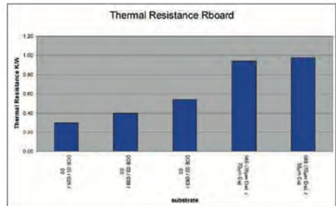
Figure 9: Simulated thermal resistance including heatspreading
