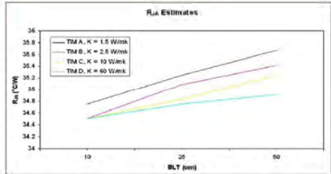
Figure 5: The impact of TIMs on RJA
