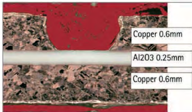
Figure 16: Thin alumina substrate with thick copper
