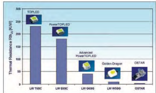
Figure 9: Trend in package thermal performance
