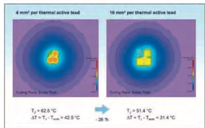
Figure 10: Influence of solder pad area
