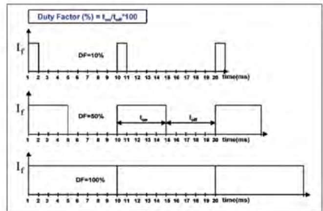
Figure 14: PWM as a method of dimming LEDs
