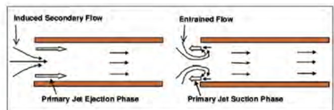
Figure 2: Operation of Synthetic jet ejector
