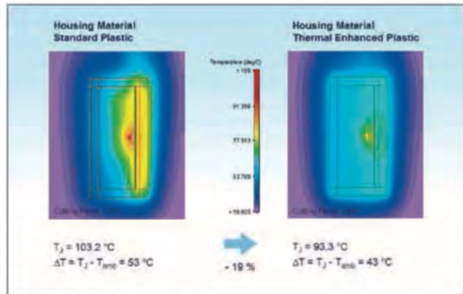
Figure 16: Thermal Impact of the housing material
