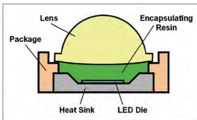
Figure 3: Cross-Section of Power LED
