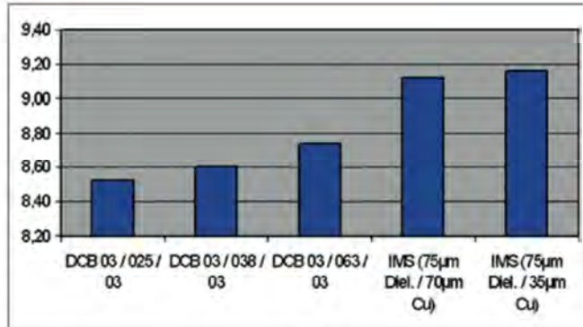
Figure 11: Overall thermal resistance junction to board (RJ-S+RS-B) in K/W
