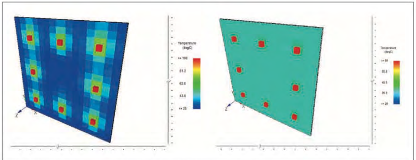
Figure 2: Calculated result of 8 LEDs each of 0.2\text{ W} of thermal loss (left) on a FR4 board ( T_J=100^\circ\text{C} ) and (right) on an IMS board ( T_J=66^\circ\text{C} )
