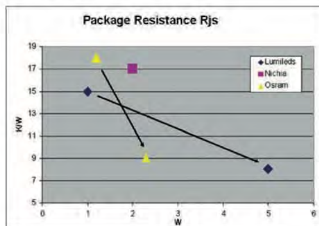
Figure 6: LED development trends for power and thermal resistance
