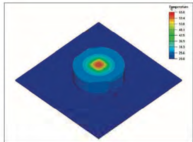
Figure 10: Overall thermal resistance junction to board (RJ-S+RS-B)
