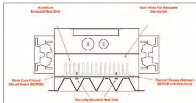
Figure 4: Gallium GS6 LED Luminaire
