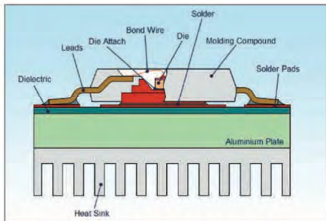
Figure 5: Internal Structure of Golden DRAGON® LED Package
