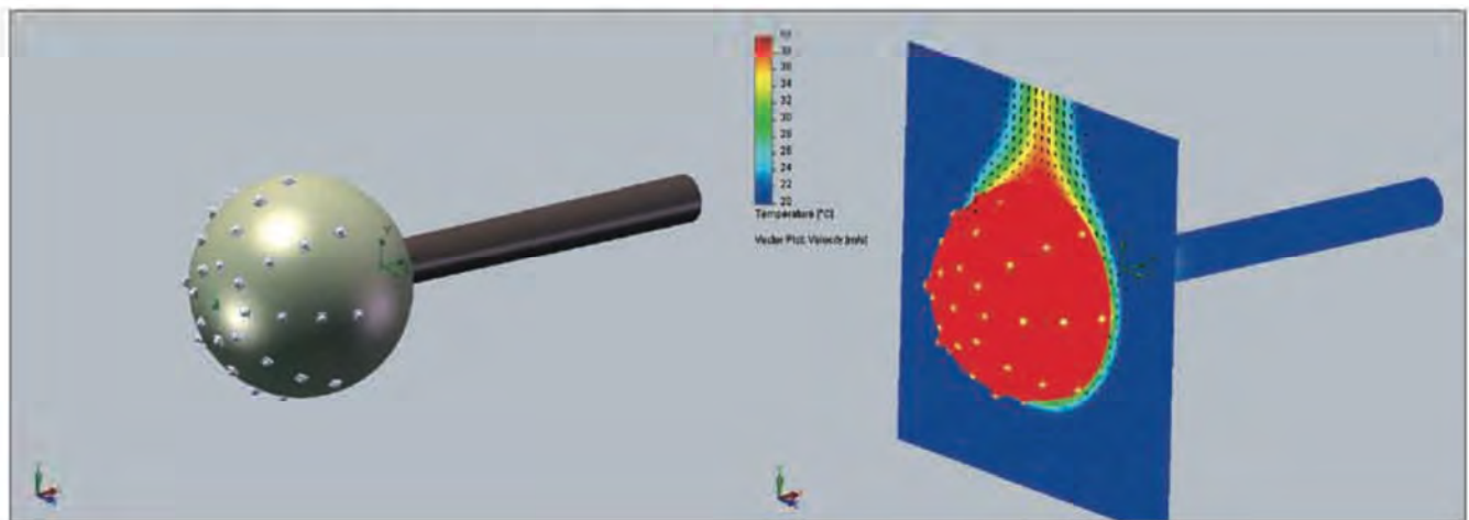
Figure 5: 33 LEDs on a spherical shell of aluminium with FR4 isolation. Internal, external airflow and heat transfer is calculated.
