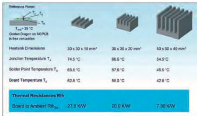
Figure 15: Thermal Resistance R_{thBA} of different heat sinks
