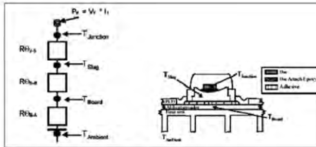
Figure 7: Model of thermal resistance, Lumileds AB05
