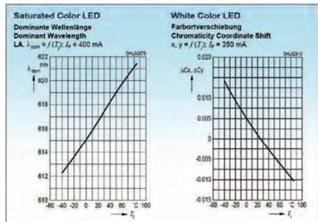
Figure 3: Example of junction temperature influence on Dominant Wavelength and Color Coordinates
