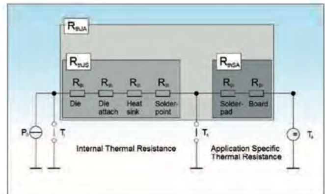
Figure 6: Static Equivalent Circuit
