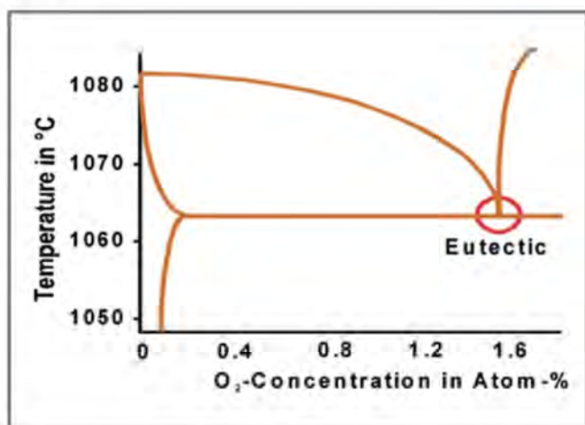
Figure 1: Eutectic of oxygen and copperoxide
