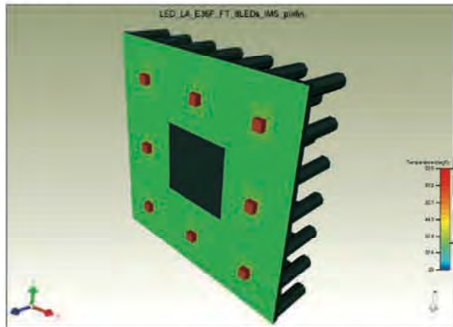
Figure 3: Calculated surface temperatures for an ambient temperature of 25 °C with 7x7 staggered pin fins each 15 mm high in free convection ("still air"). Temperature drops to T_J = 63 °C, only. If this doesn't seem to be sufficient, FLOTHERM can look for a better solution by Design of Experiments (DOE) and subsequent optimization steps.
