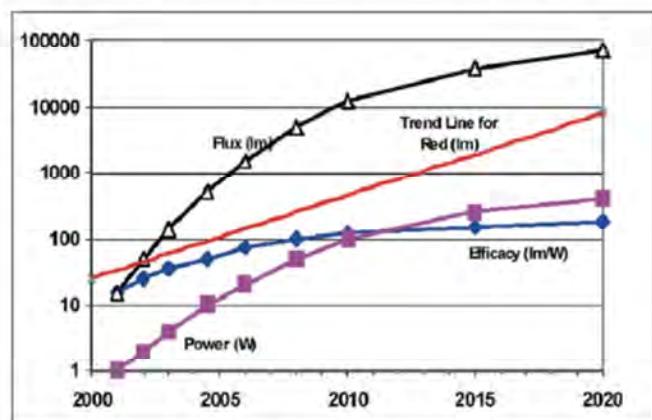
Figure 4: Expected development of LED power, Shatli [4]
