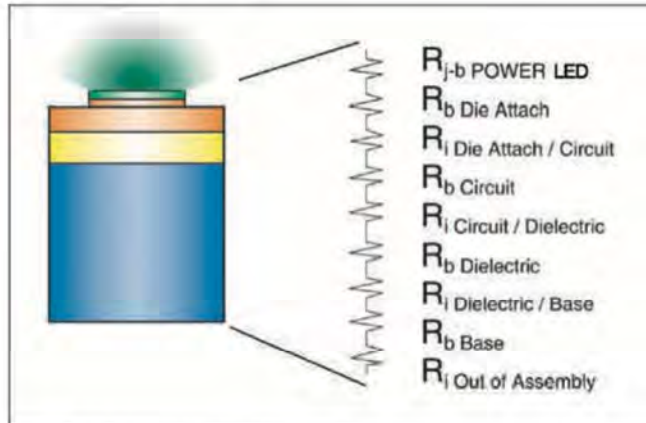
Figure 1: Thermal resistances in a HB-LED lighting assembly.
