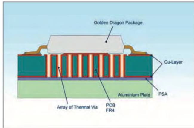
Figure 12: Principle Design of FR4 with thermal vias
