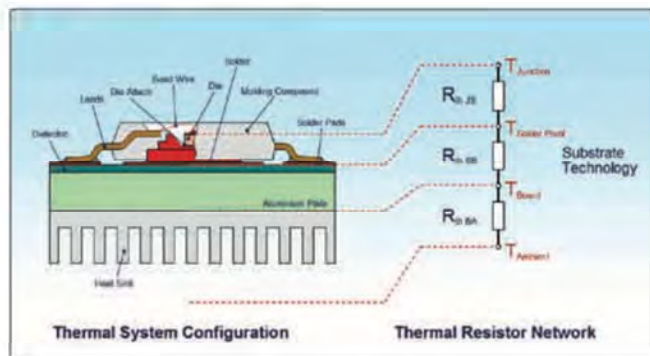
Figure 7: Resistances Serial Configuration
