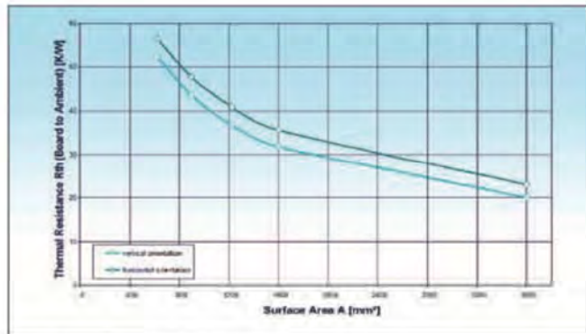
Figure 14: Thermal Resistance R_{thBA} vs. Substrate Area
