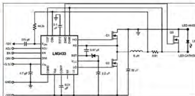
LM3433 Block Diagram
