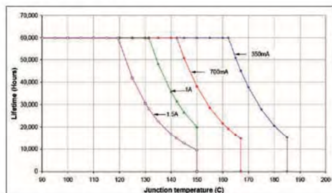
Figure 6. Lifetimes across current and temperature variables.
