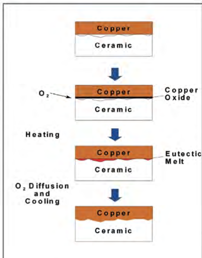
Figure 2: DCB-Process
