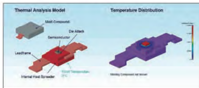
Figure 8: Internal Thermal Resistance R_{thJS}
