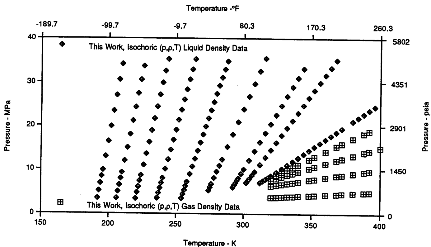
Figure 41. Range of Measured Temperatures and Pressures for Isochoric (p,ρ,T) Data for a Mixture of R41/744 with x(\text{R41}) = 0.49982 Mole Fraction (0.43591 Mass Fraction).
