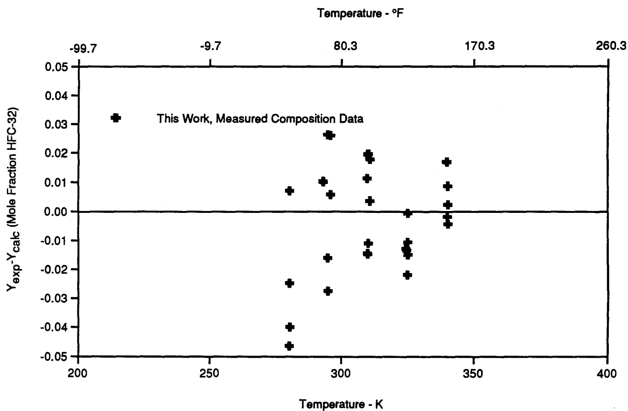
Figure 25. Comparison of Vapor Compositions for the R32/290 System; the Baseline is from the Lemmon-Jacobsen Model in REFPROP 6.0.
