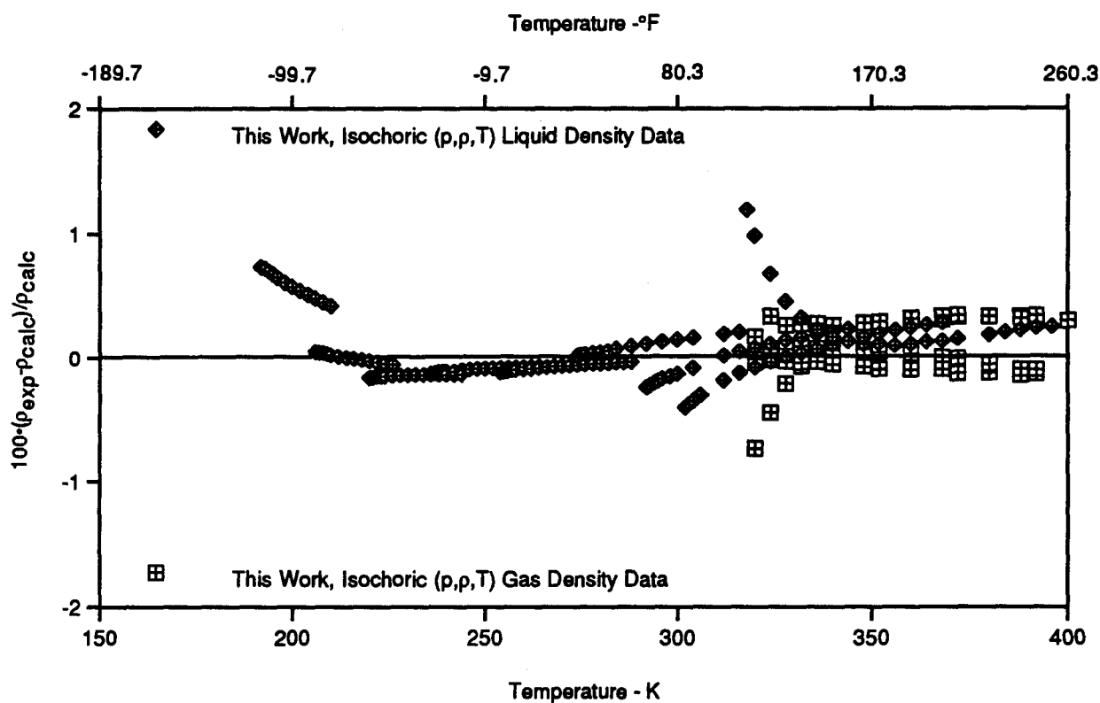
Figure 42. Comparison of Isochoric (p,ρ,T) Data for the Equimolar Mixture of R41/744; the Baseline is from the Lemmon-Jacobsen Model in REFPROP 6.0.
