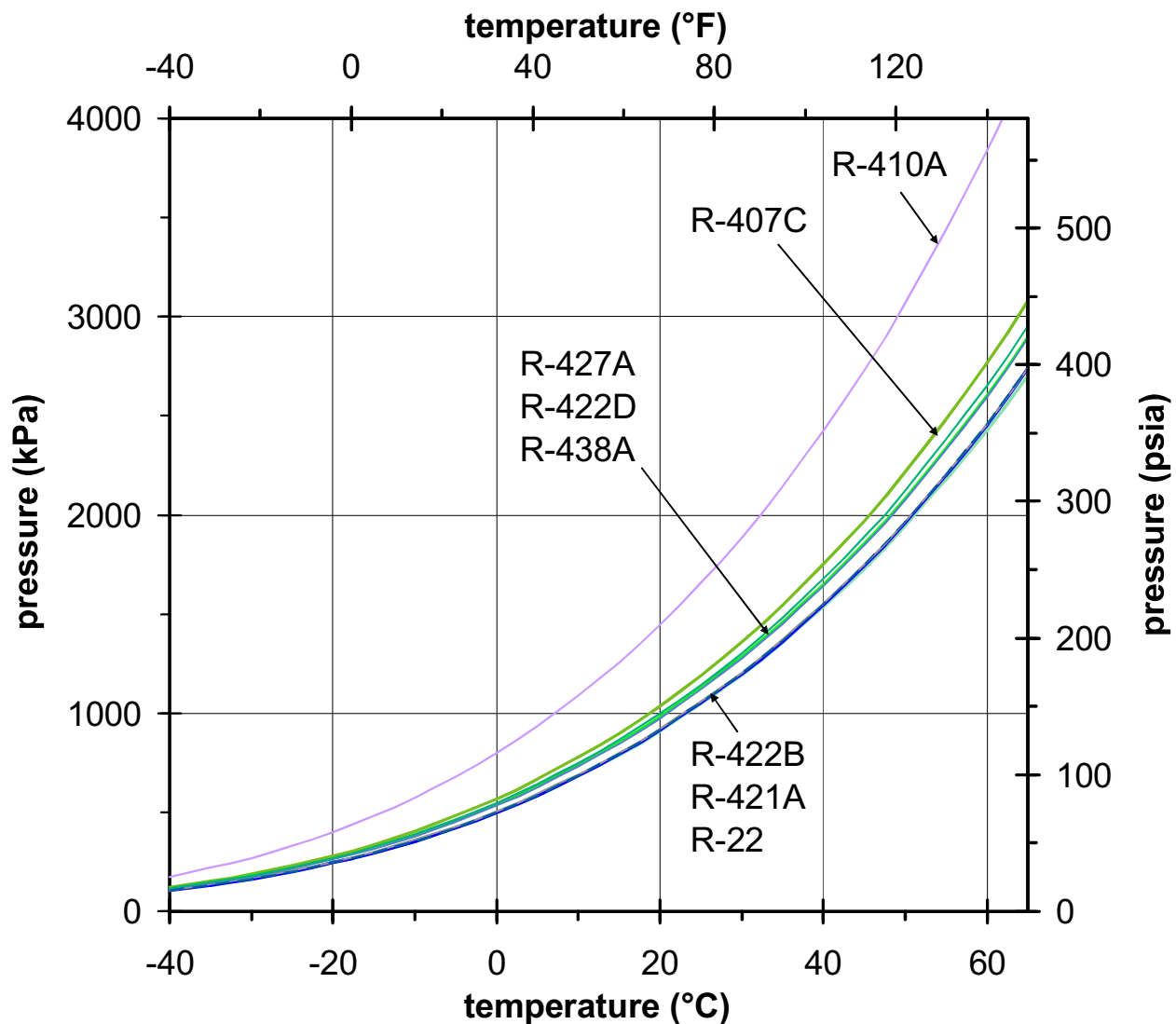
Figure 1: Pressure-Temperature Comparison
