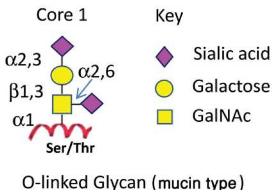
Figure 3. O-linked glycans.
