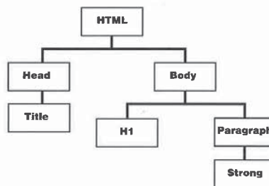
Figure 7-1. Containment relationships between the elements in an HTML document.
