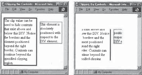
Figure 12-4. A DIV element with part of its contents outside its borders, with no clipping (on the left) and with a clipping rectangle defined (on the right).
