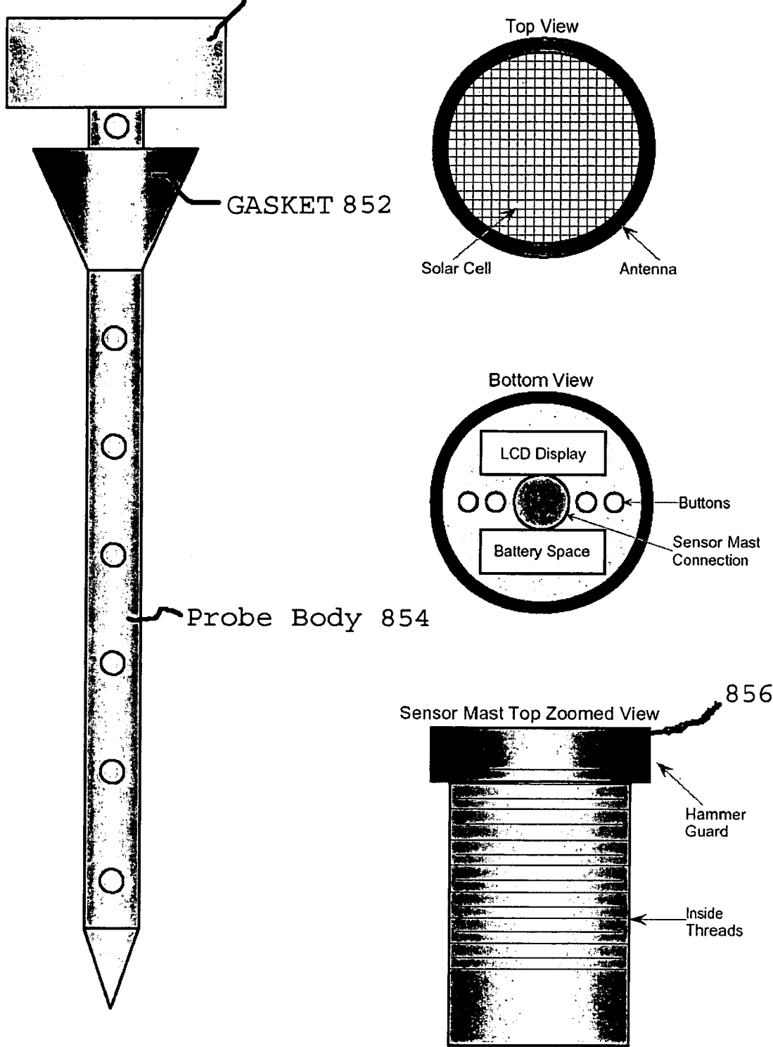
Figure 8 - Separable Probe Body TOP PART 850
