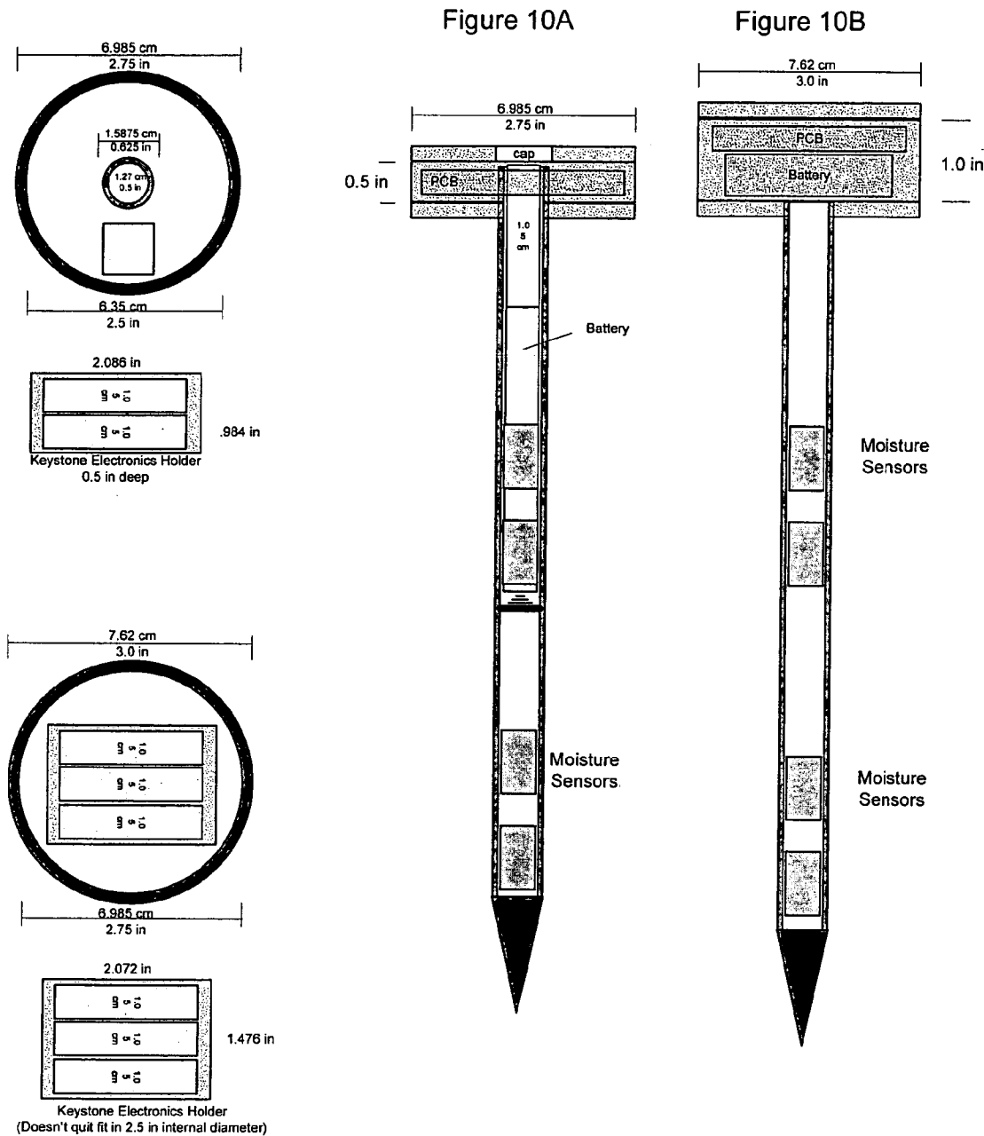
Figure 10 - Configuration and Dimensions of Probe Body
