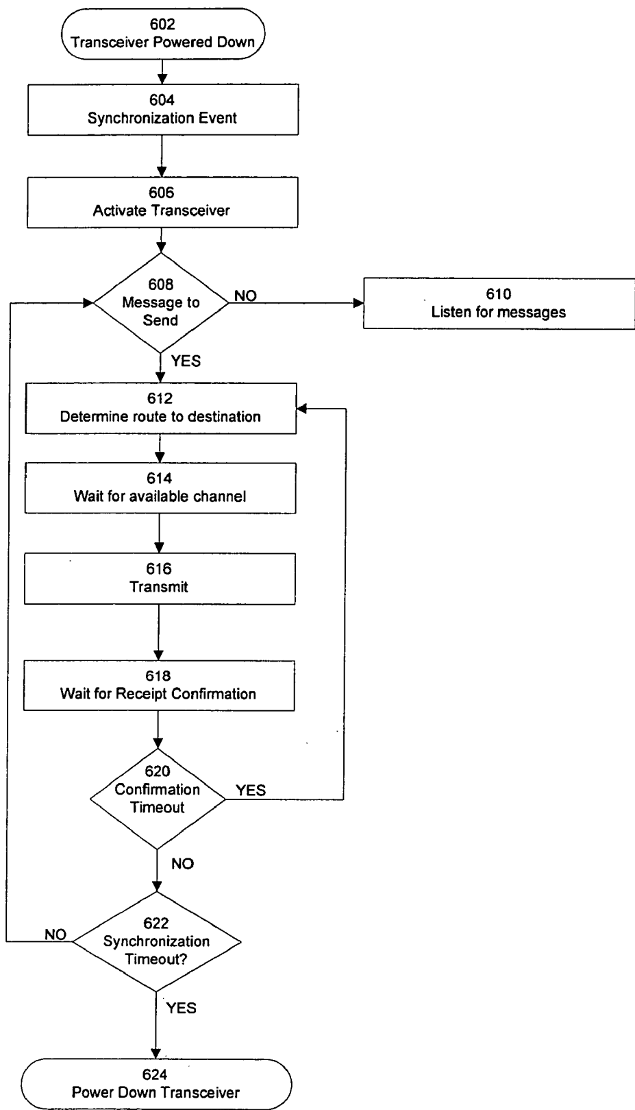
Figure 6 - Transceiver Synchronization
